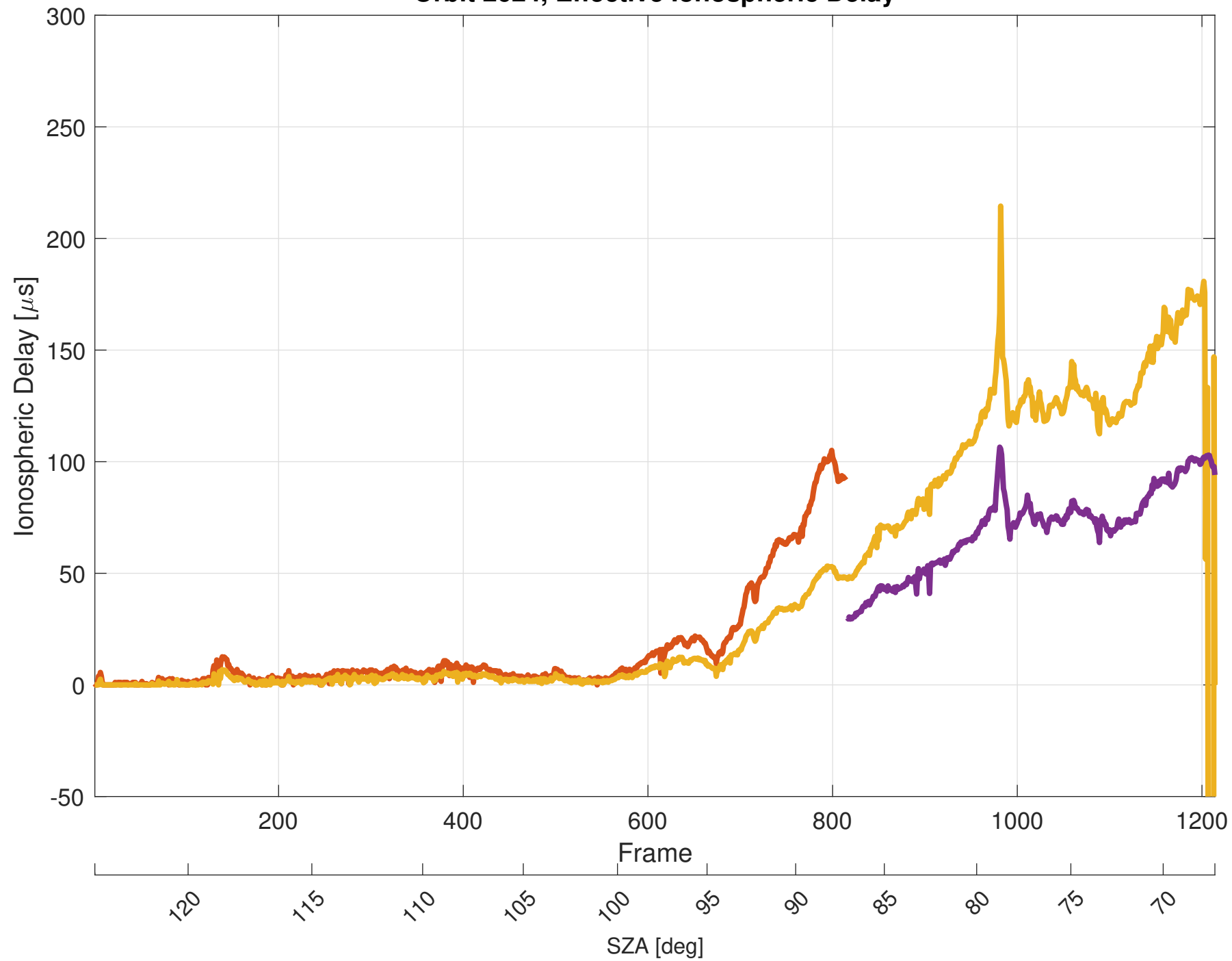
Orbit 2624, Effective Ionospheric Delay
