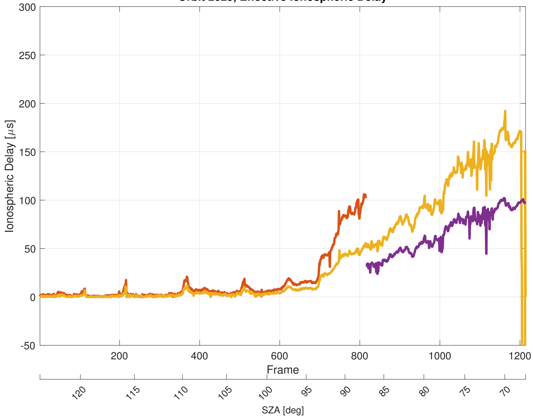
Orbit 2625, Effective Ionospheric Delay
