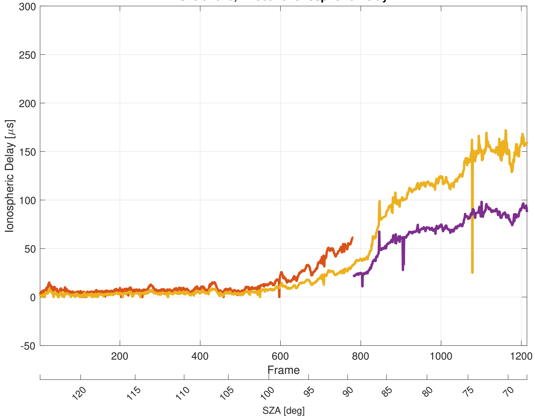
Orbit 2626, Effective Ionospheric Delay
