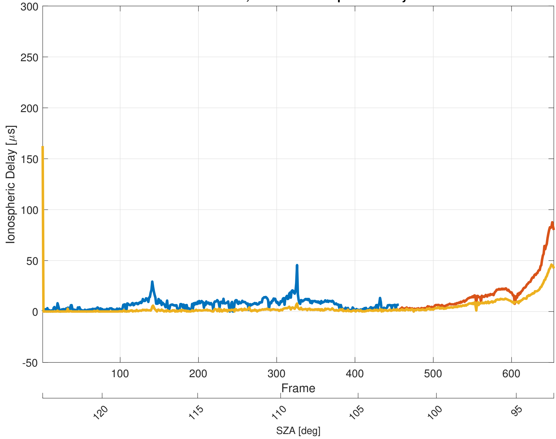
Orbit 2635, Effective Ionospheric Delay
