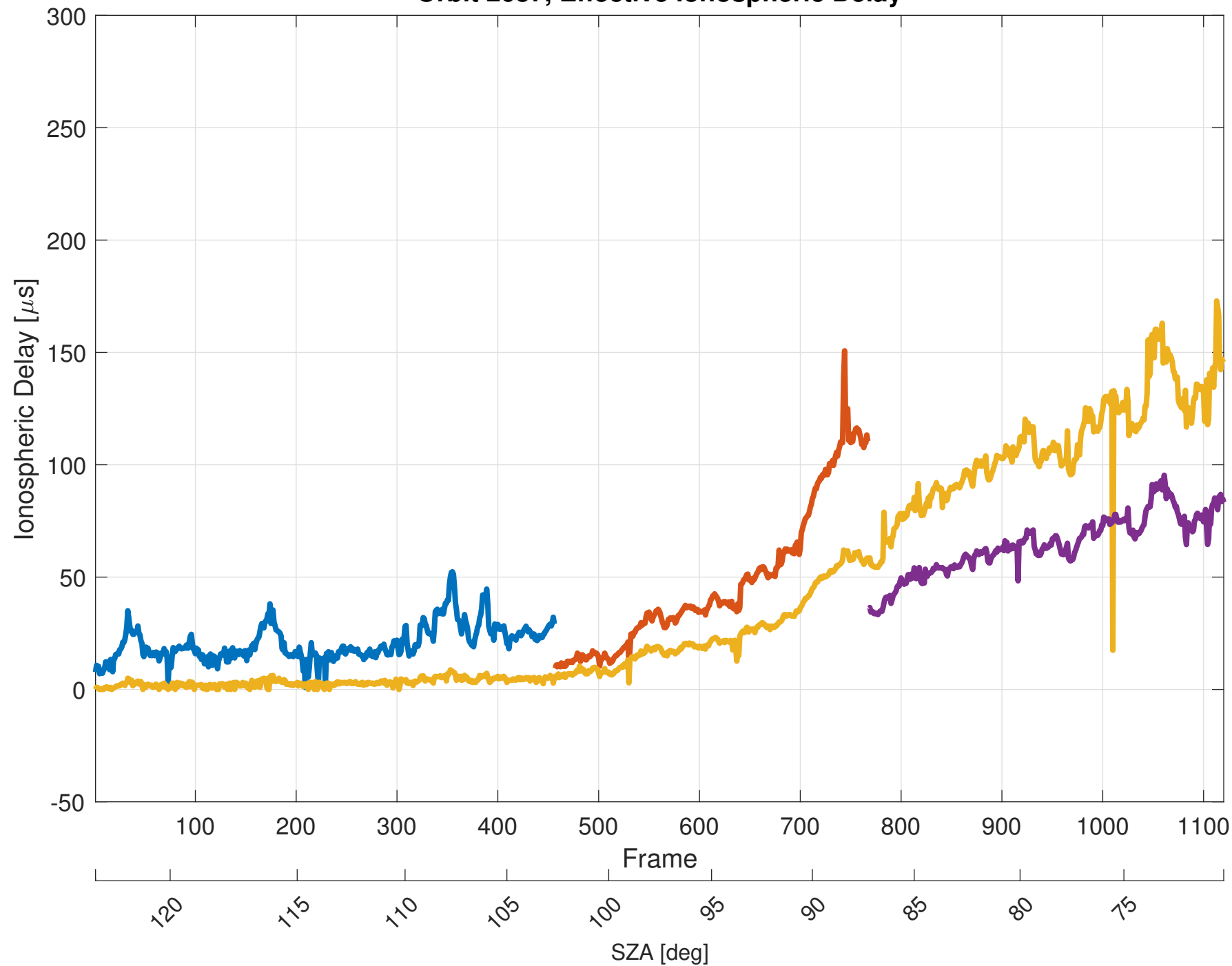
Orbit 2637, Effective Ionospheric Delay
