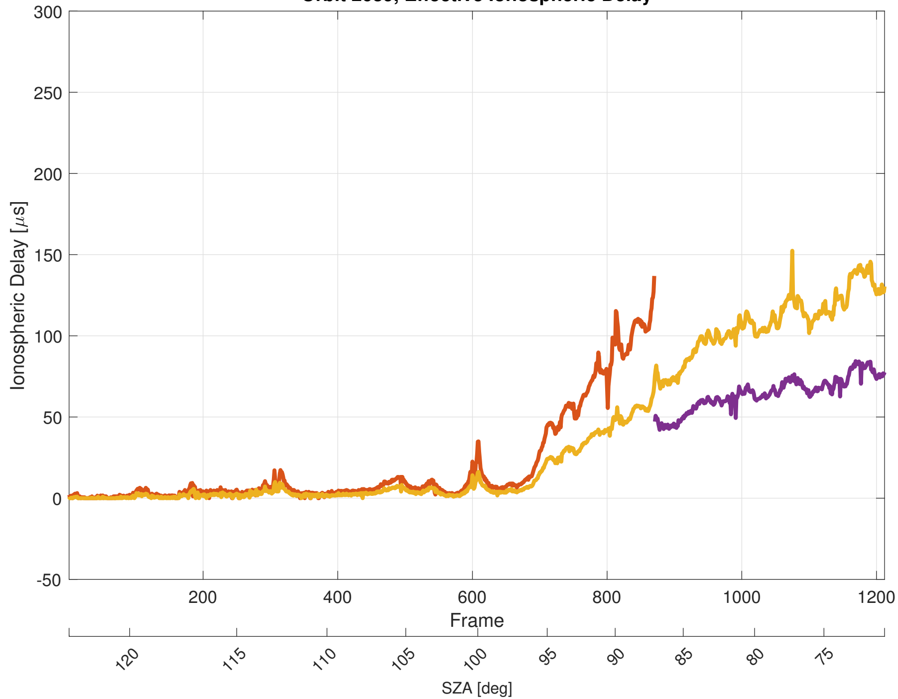
Orbit 2639, Effective Ionospheric Delay
