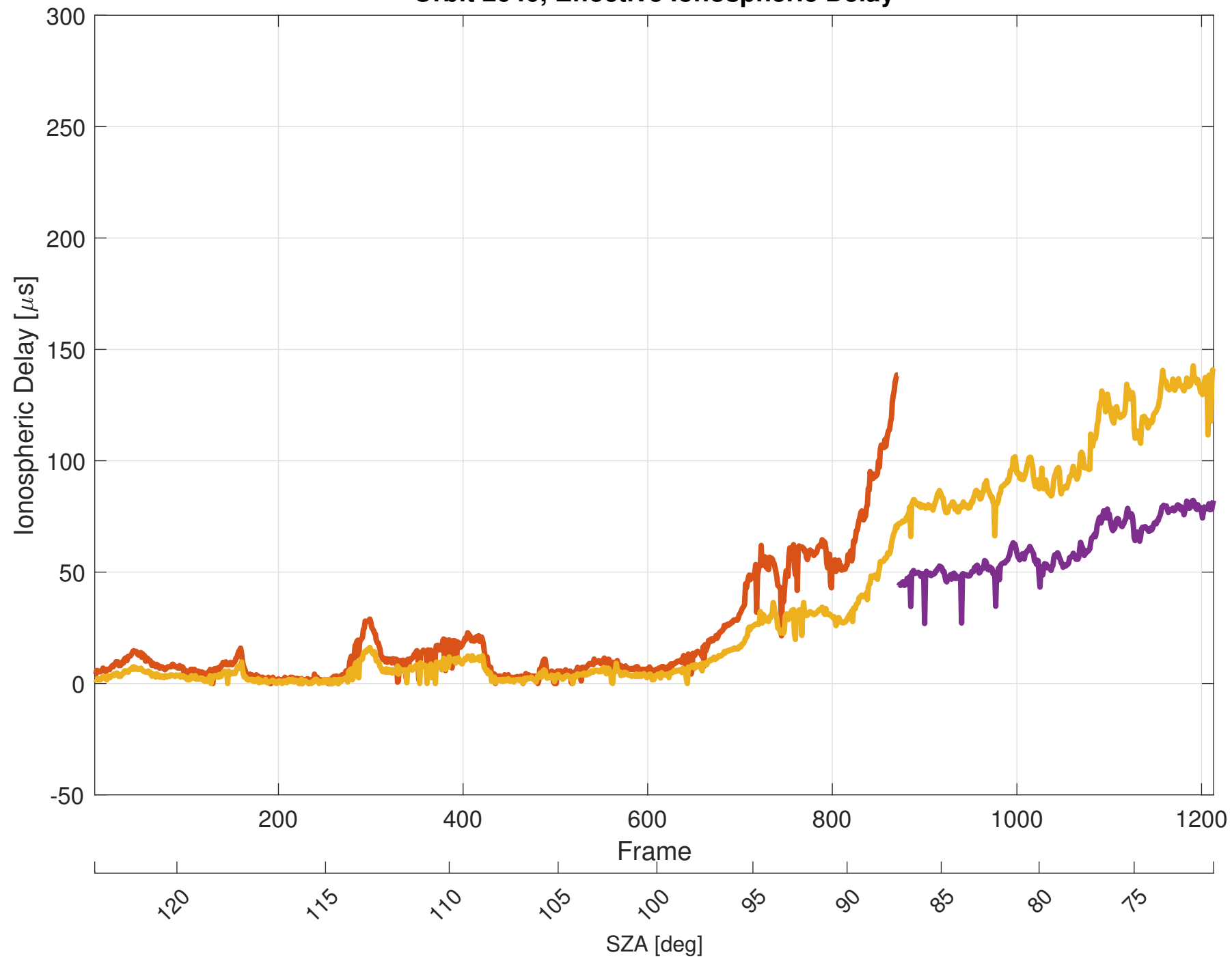
Orbit 2640, Effective Ionospheric Delay
