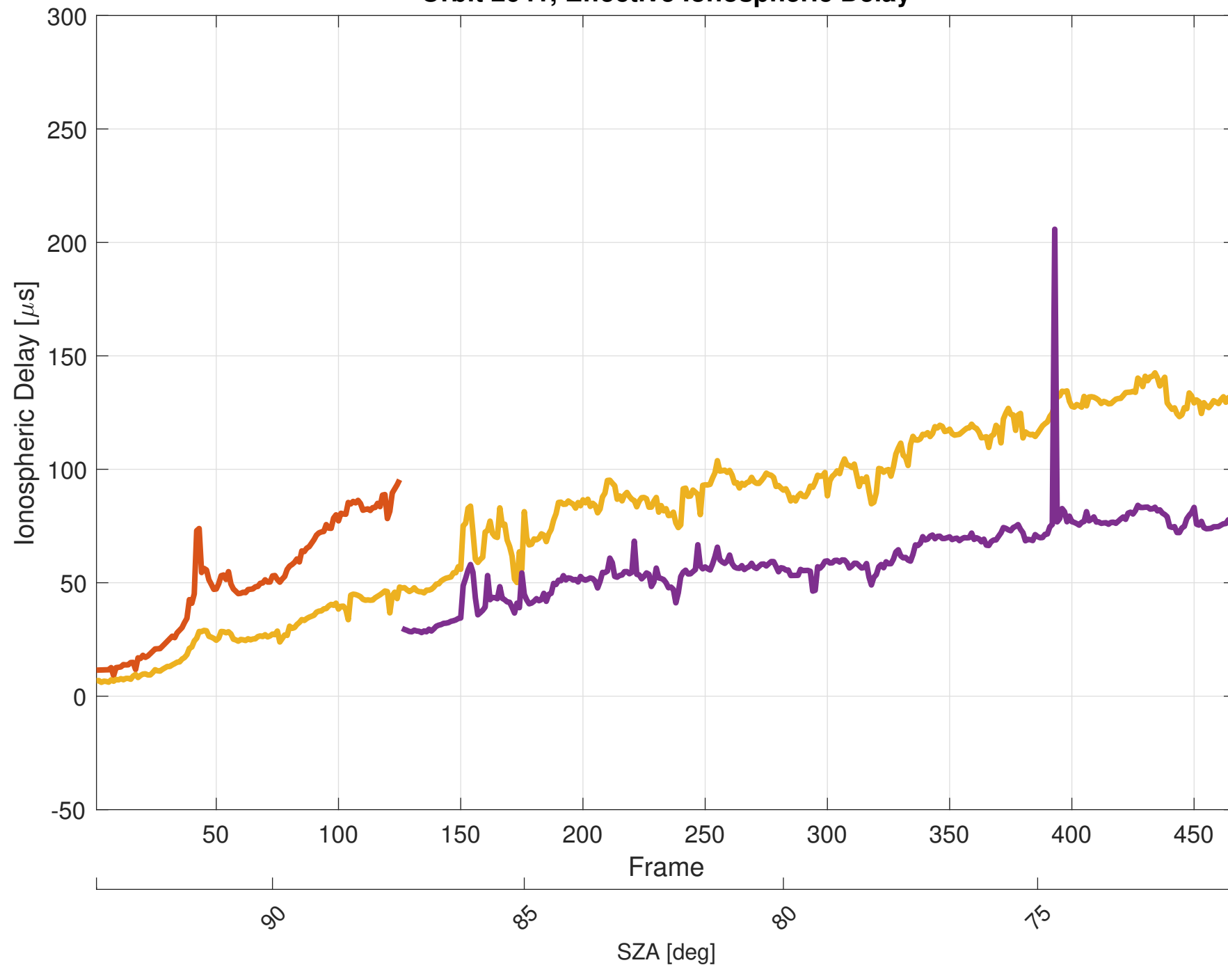
Orbit 2641, Effective Ionospheric Delay
