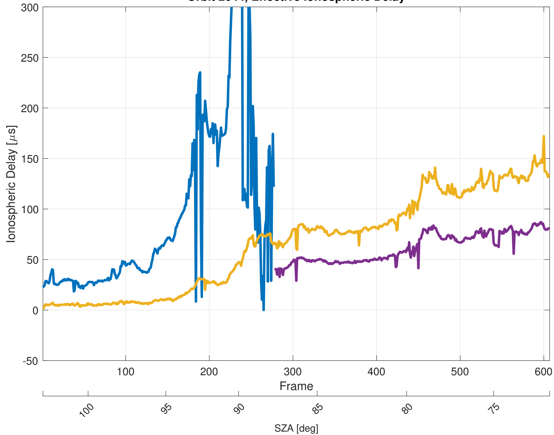
Orbit 2644, Effective Ionospheric Delay
