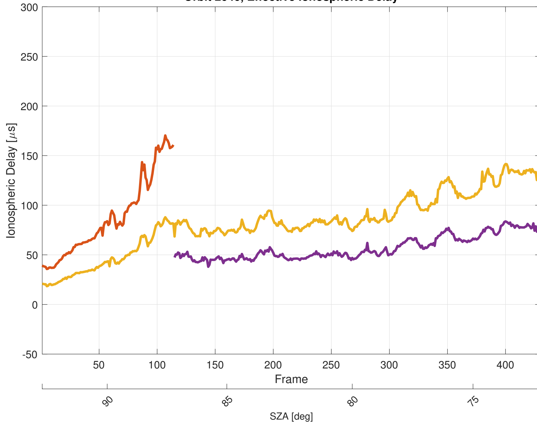
Orbit 2646, Effective Ionospheric Delay
