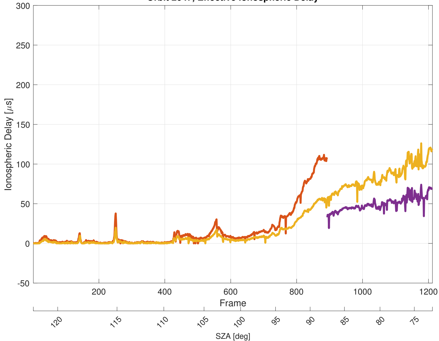
Orbit 2647, Effective Ionospheric Delay
