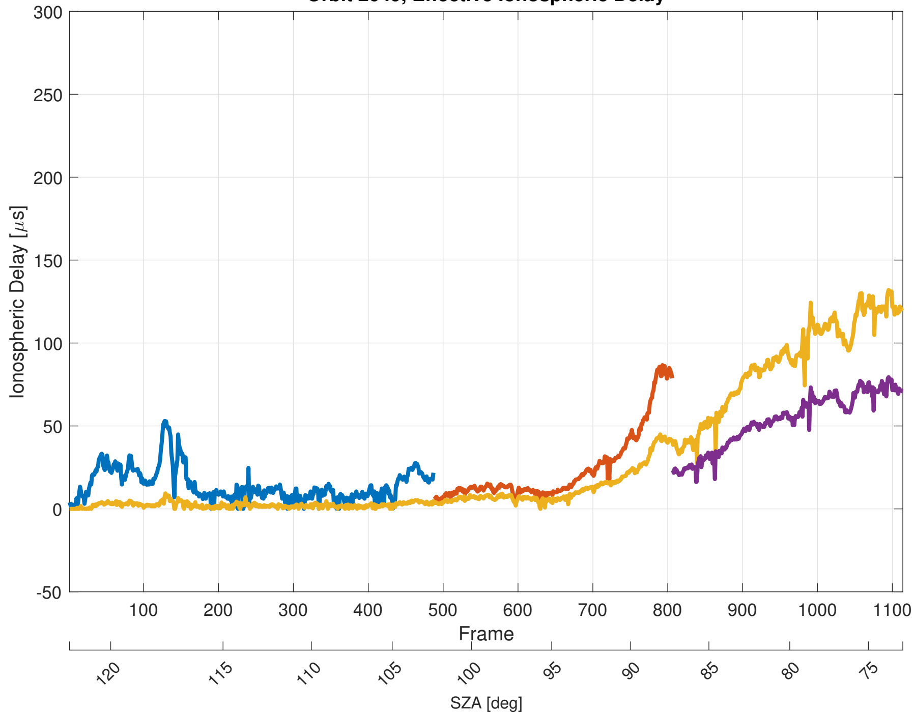
Orbit 2649, Effective Ionospheric Delay
