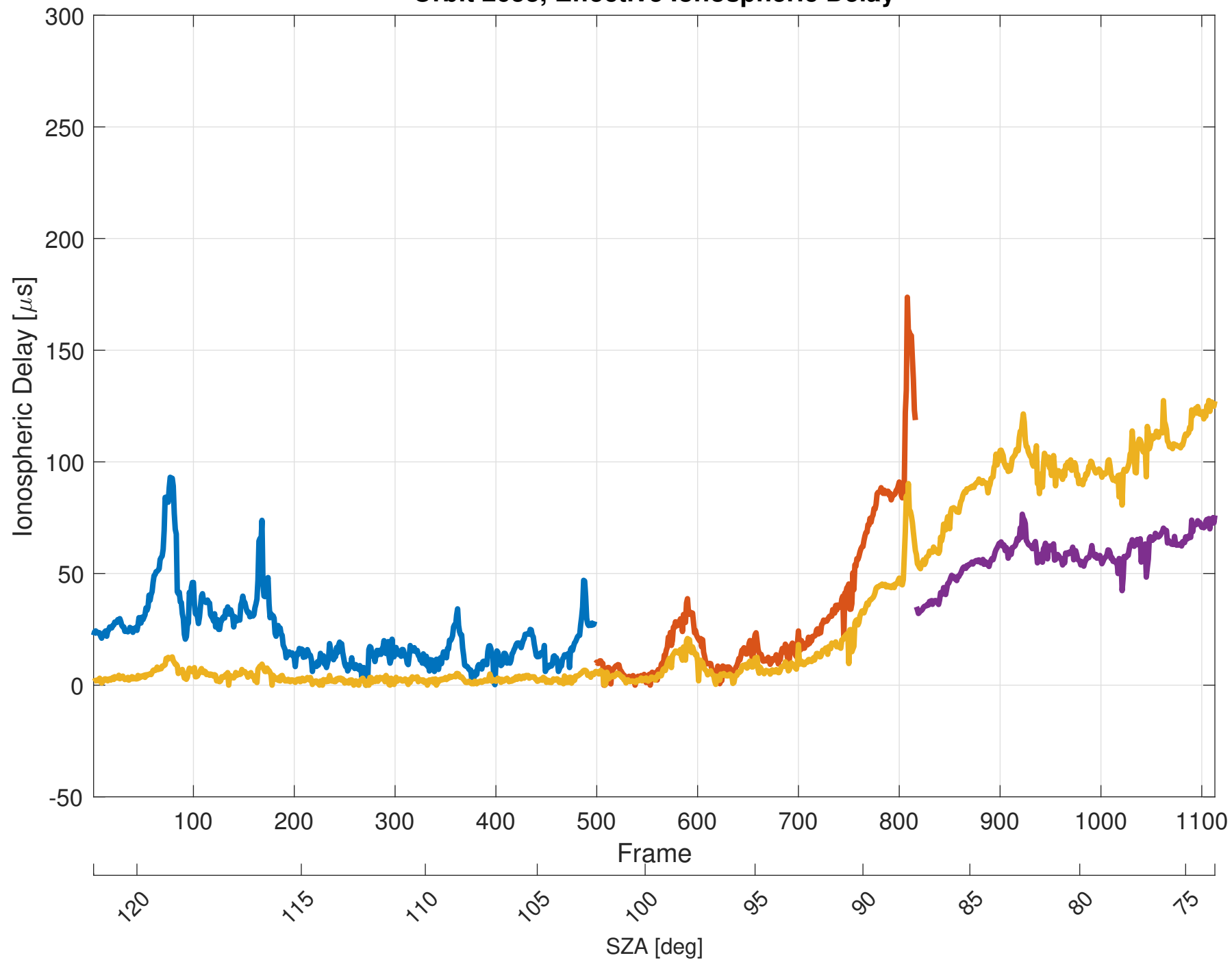
Orbit 2653, Effective Ionospheric Delay
