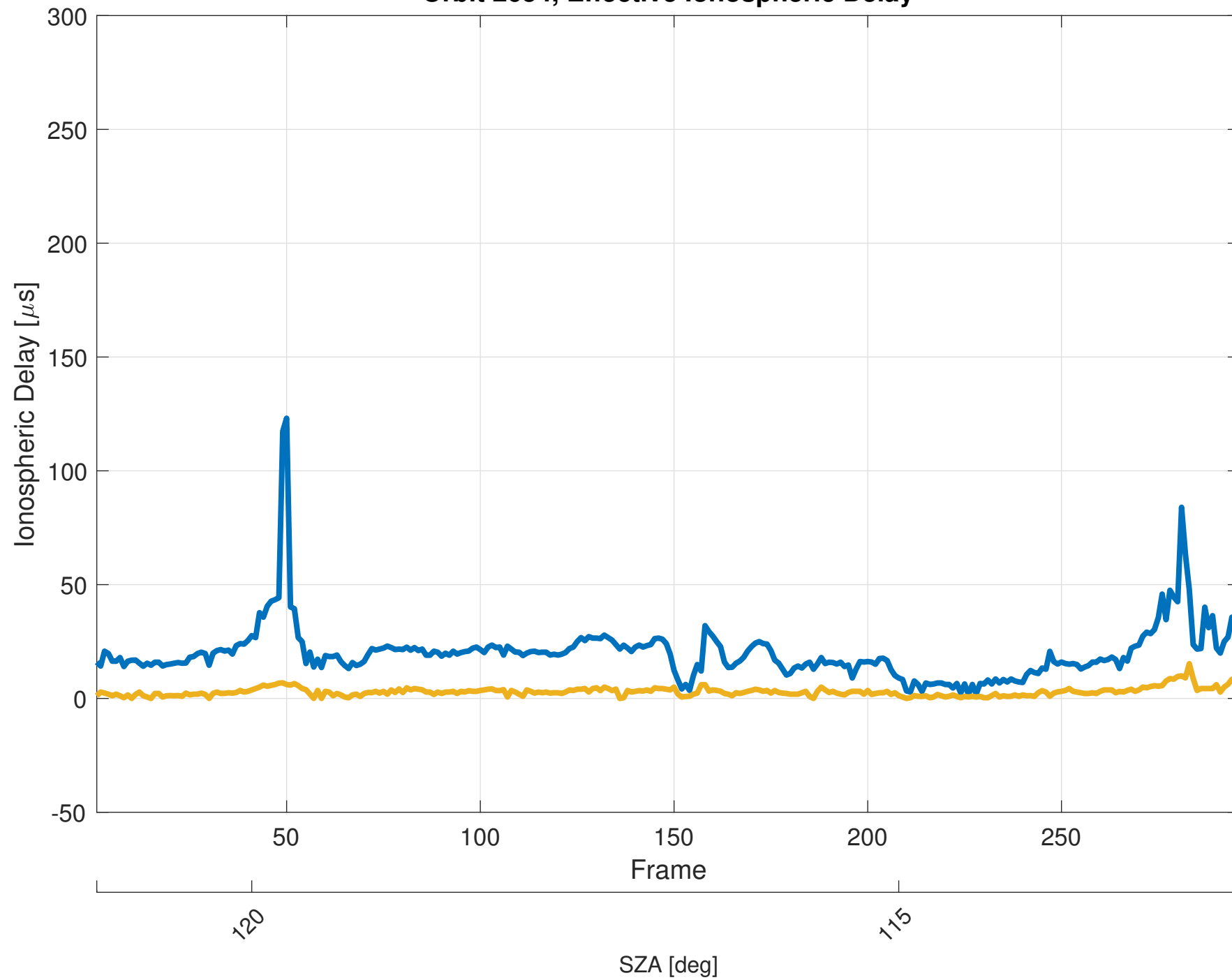
Orbit 2654, Effective Ionospheric Delay
