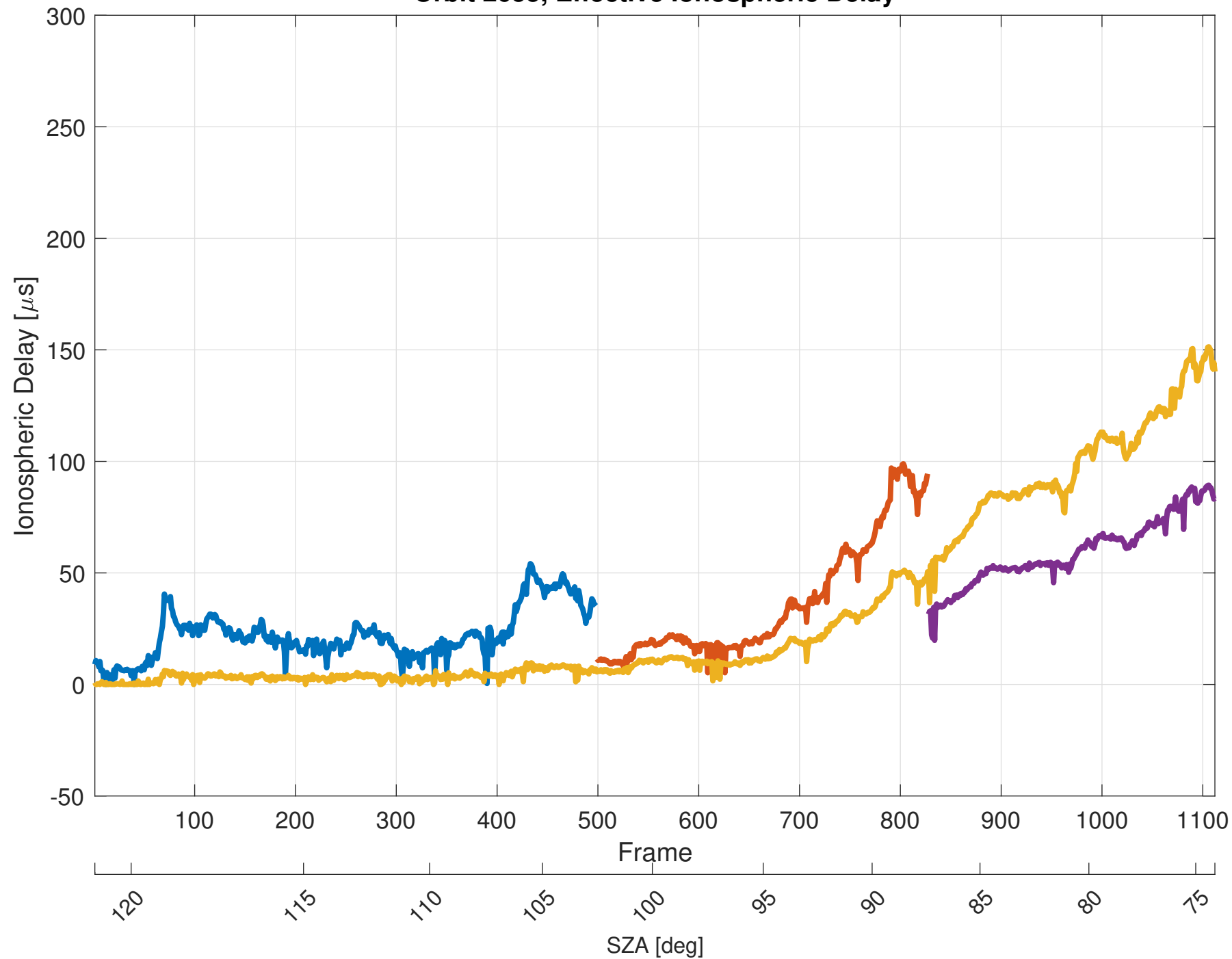
Orbit 2655, Effective Ionospheric Delay
