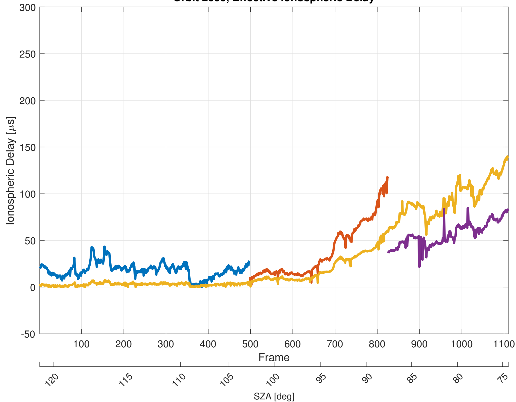
Orbit 2656, Effective Ionospheric Delay
