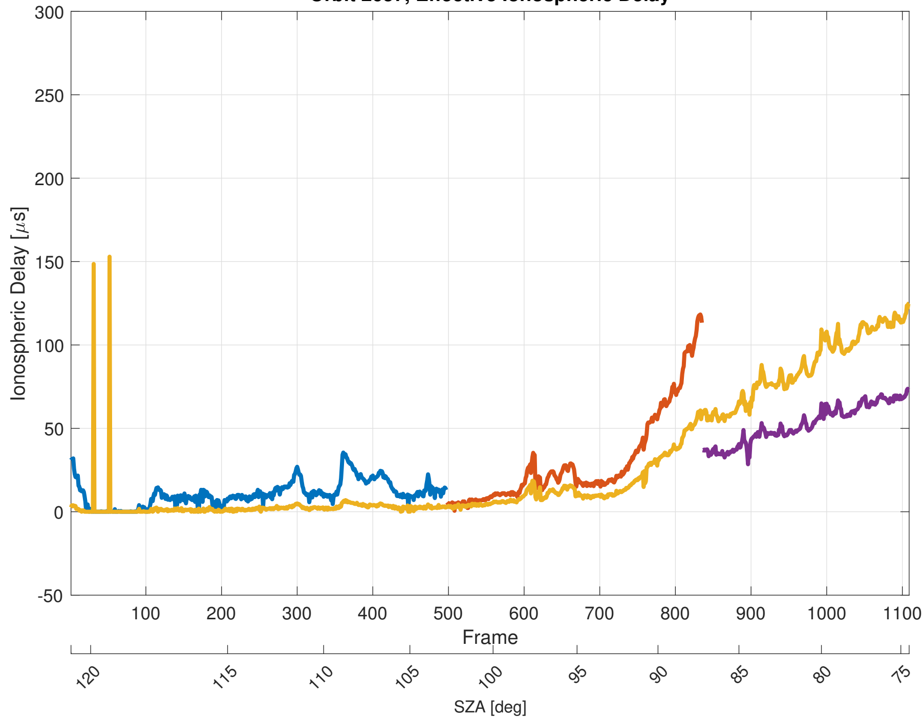
Orbit 2657, Effective Ionospheric Delay
