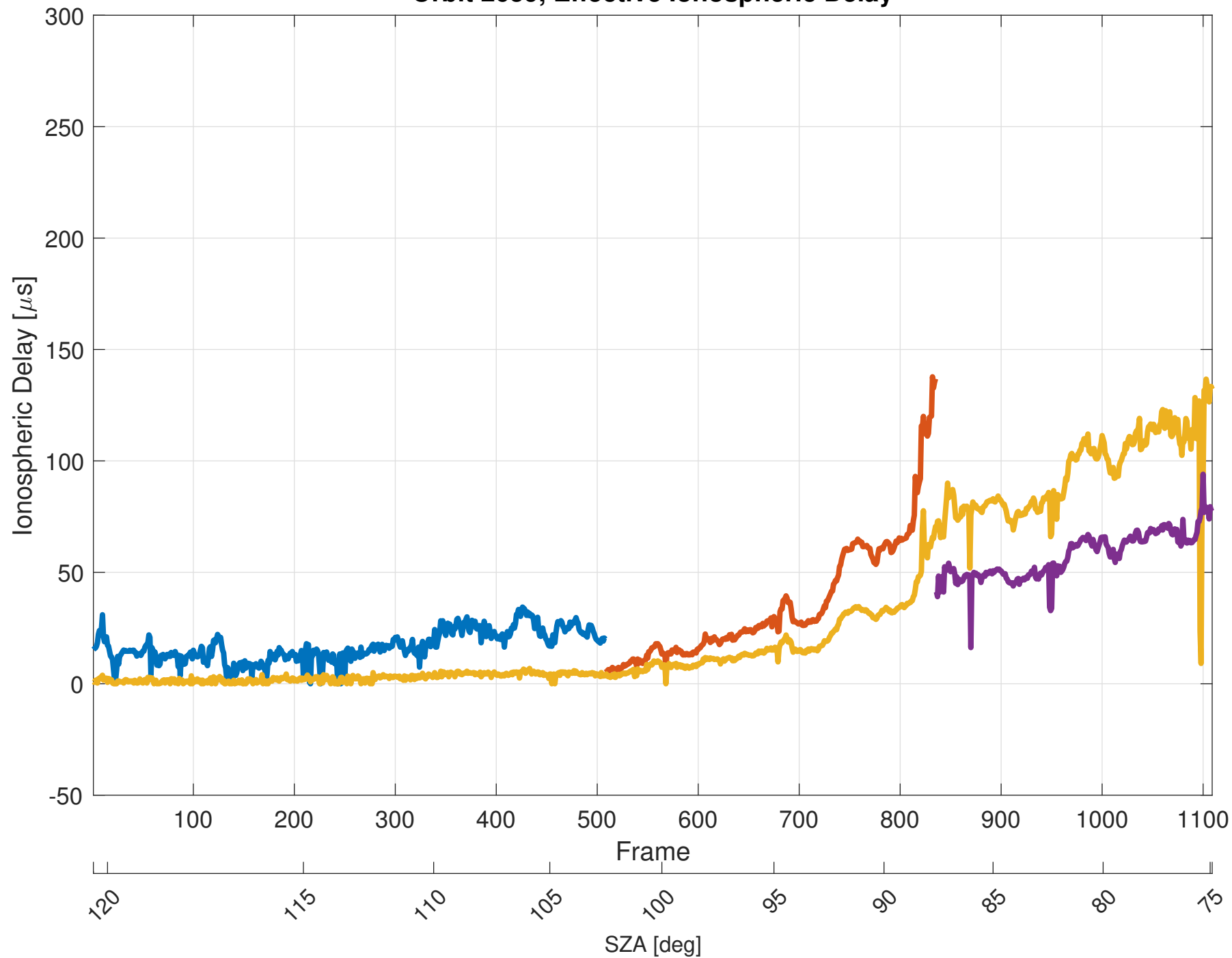
Orbit 2659, Effective Ionospheric Delay
