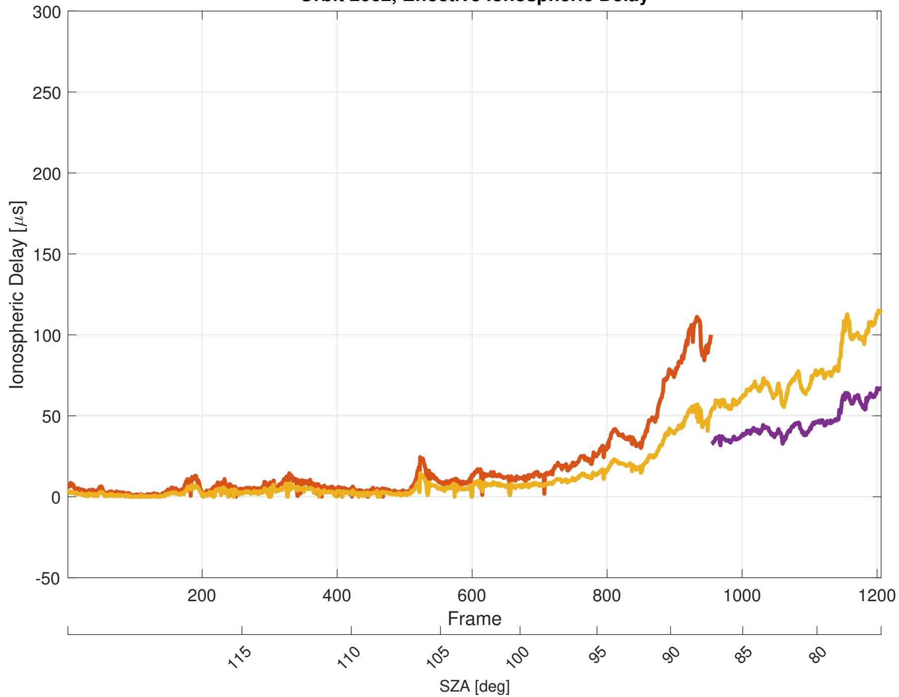
Orbit 2662, Effective Ionospheric Delay
