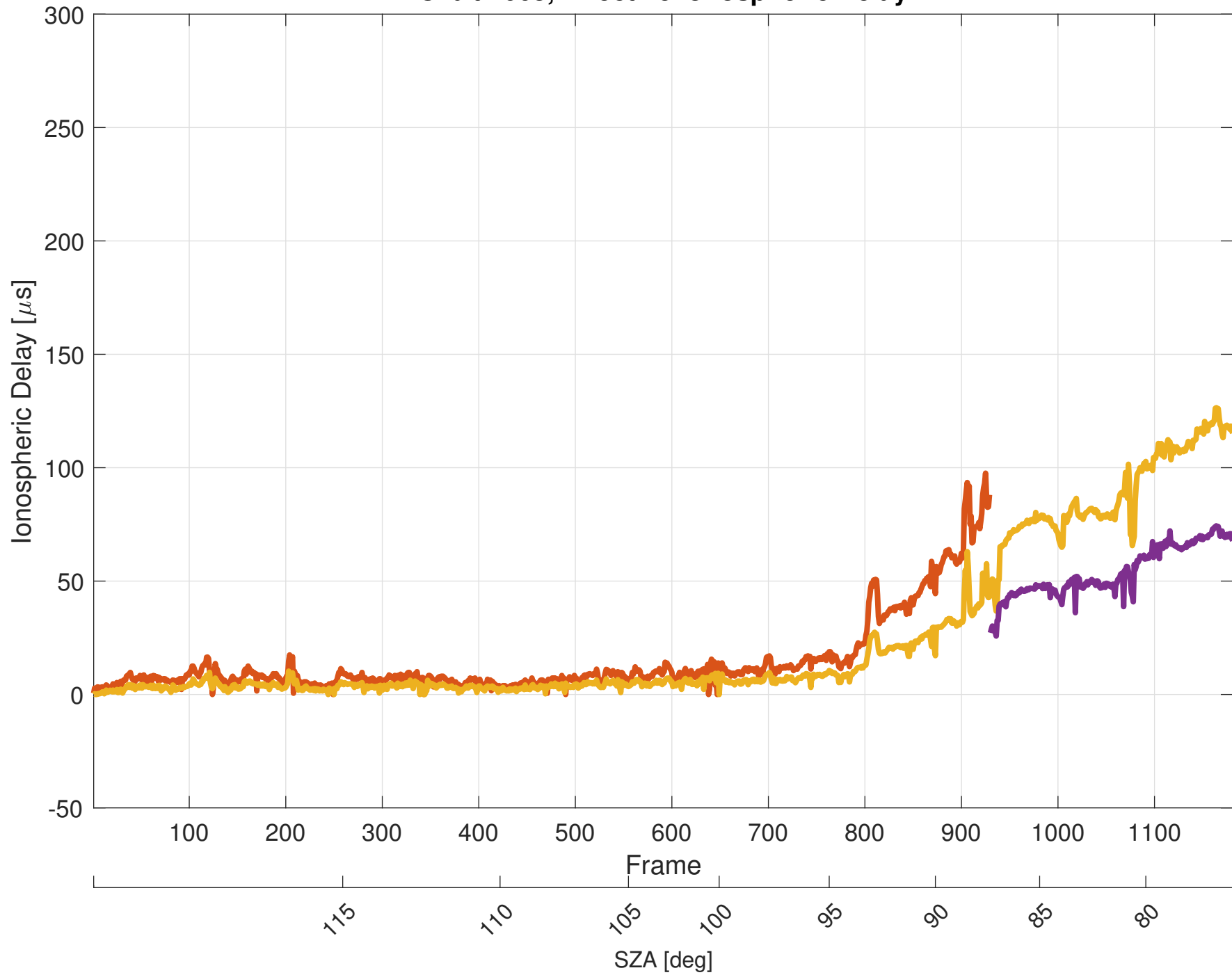
Orbit 2663, Effective Ionospheric Delay
