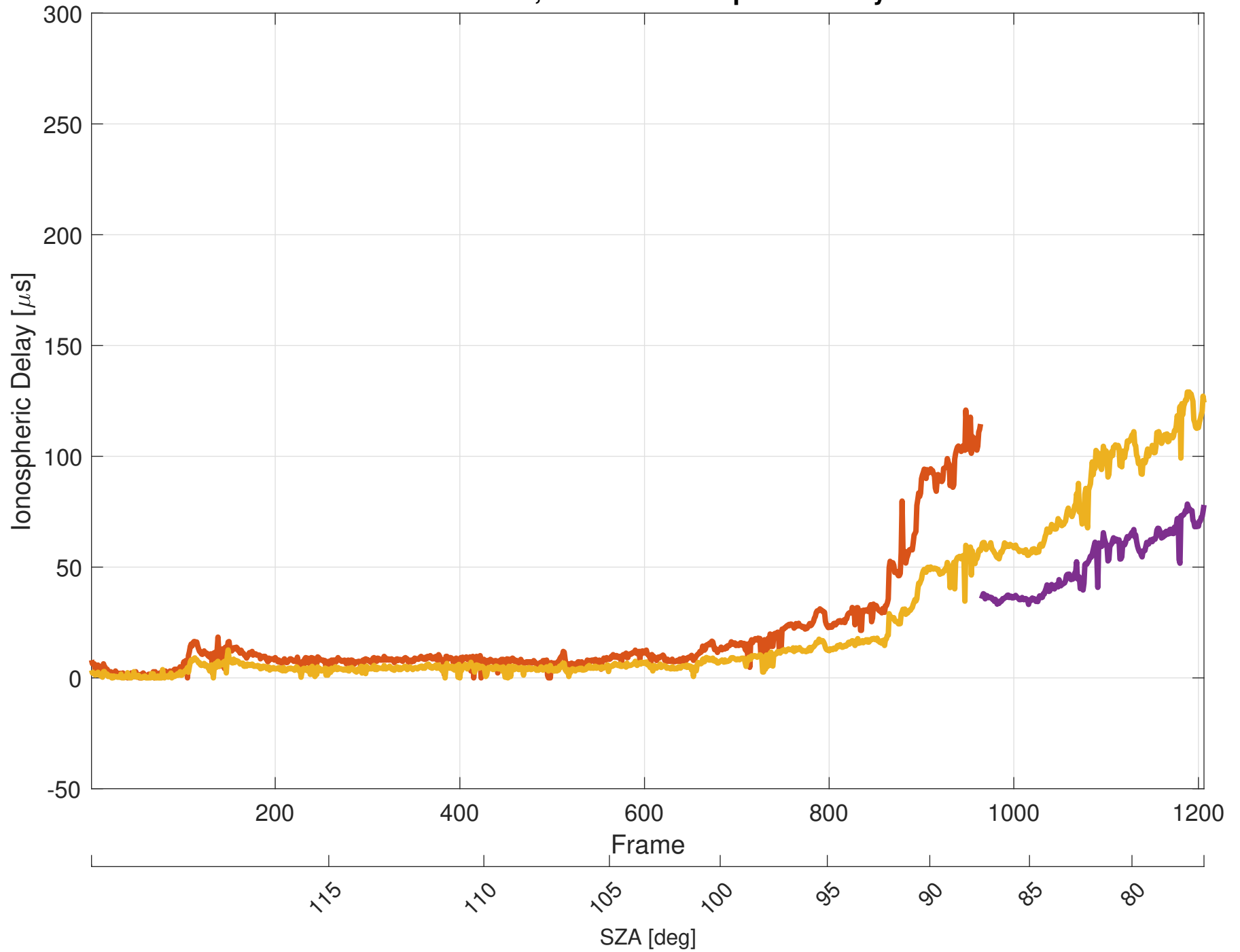
Orbit 2666, Effective Ionospheric Delay
