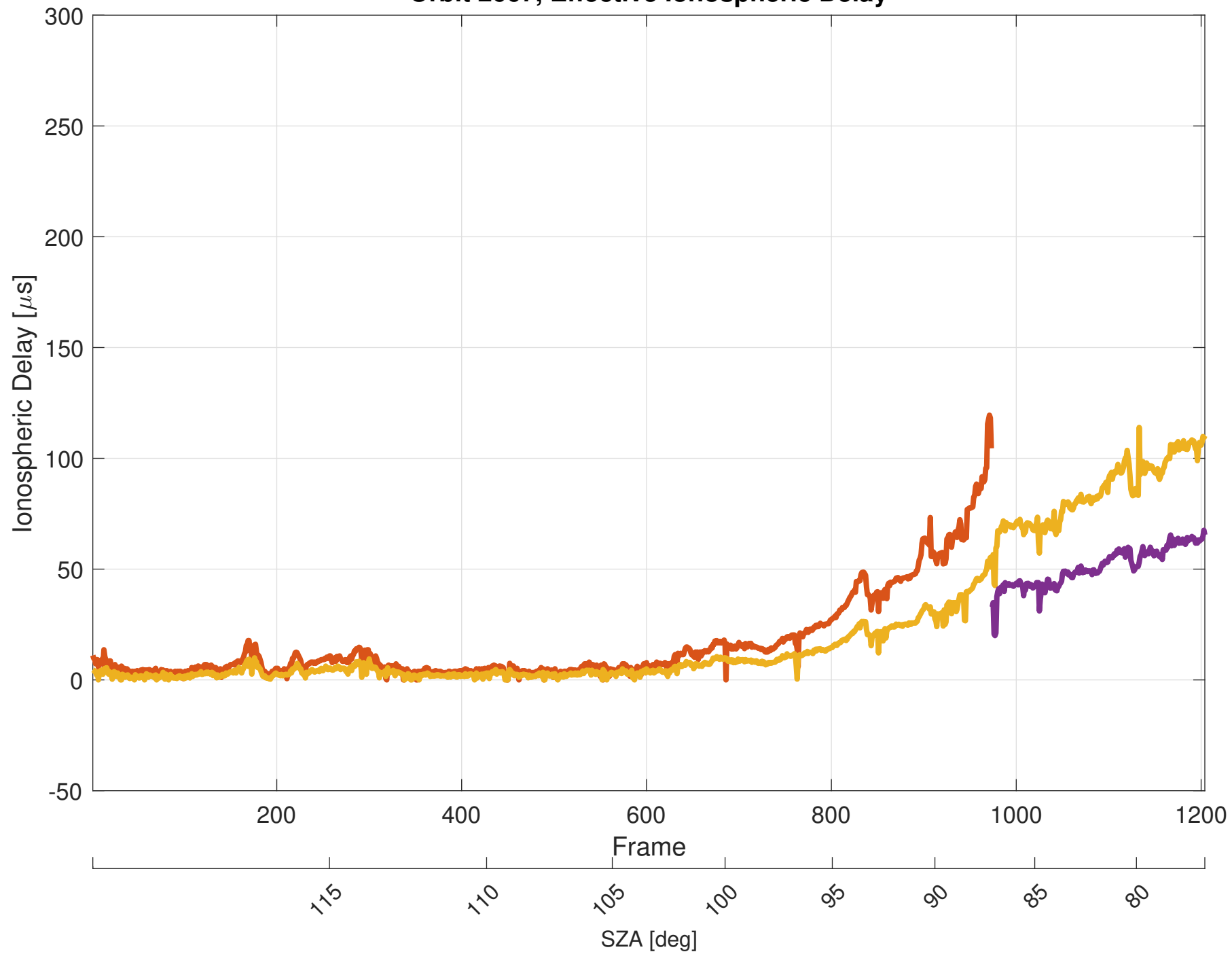
Orbit 2667, Effective Ionospheric Delay
