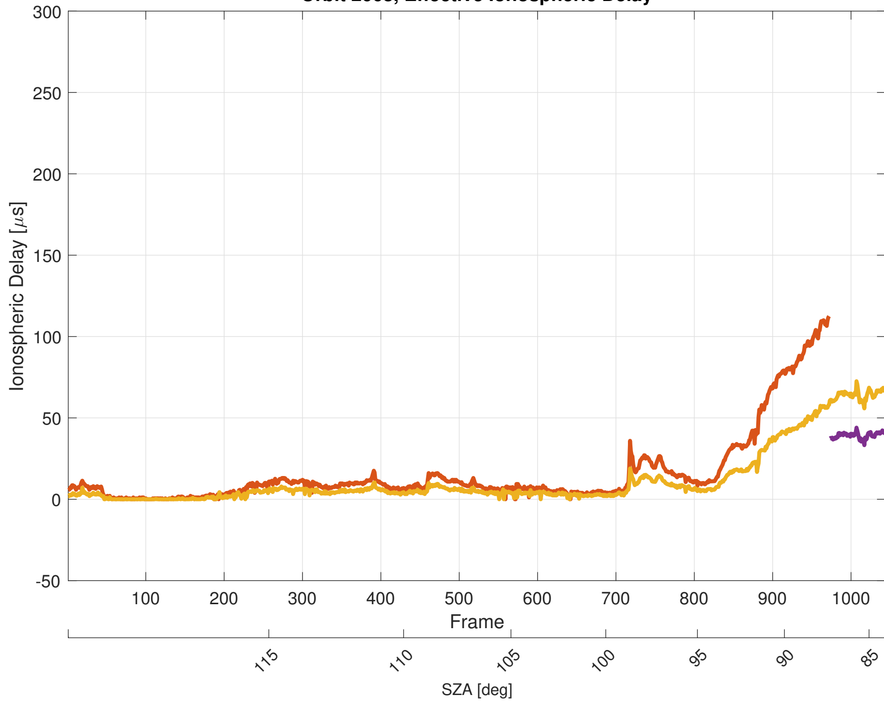
Orbit 2668, Effective Ionospheric Delay
