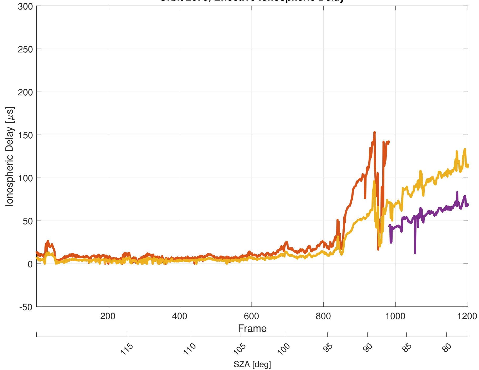
Orbit 2670, Effective Ionospheric Delay
