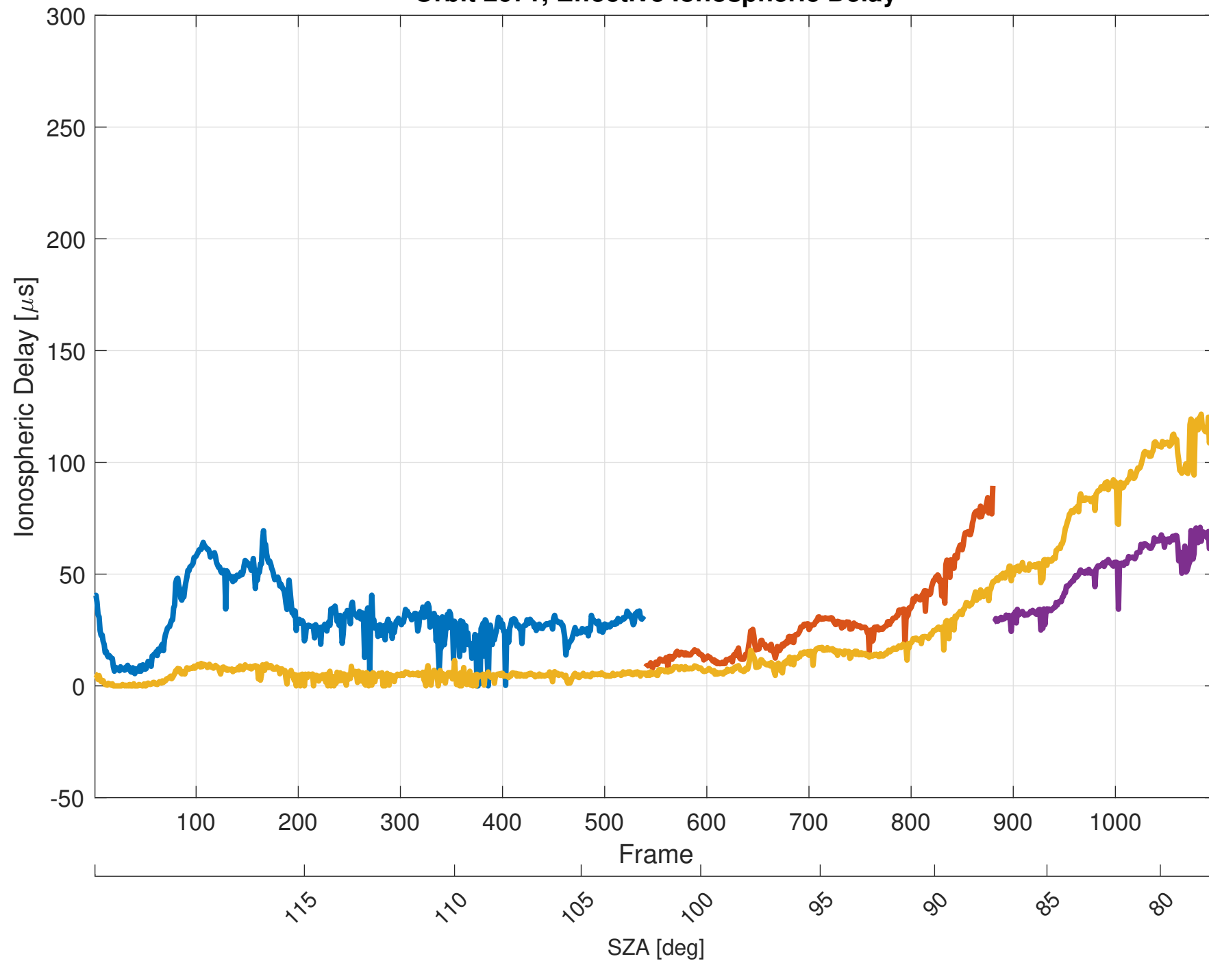
Orbit 2671, Effective Ionospheric Delay
