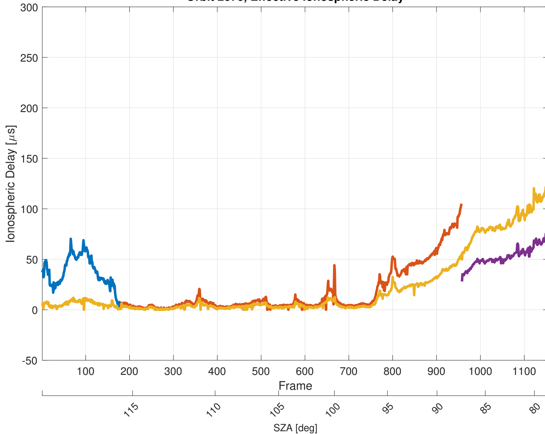
Orbit 2676, Effective Ionospheric Delay
