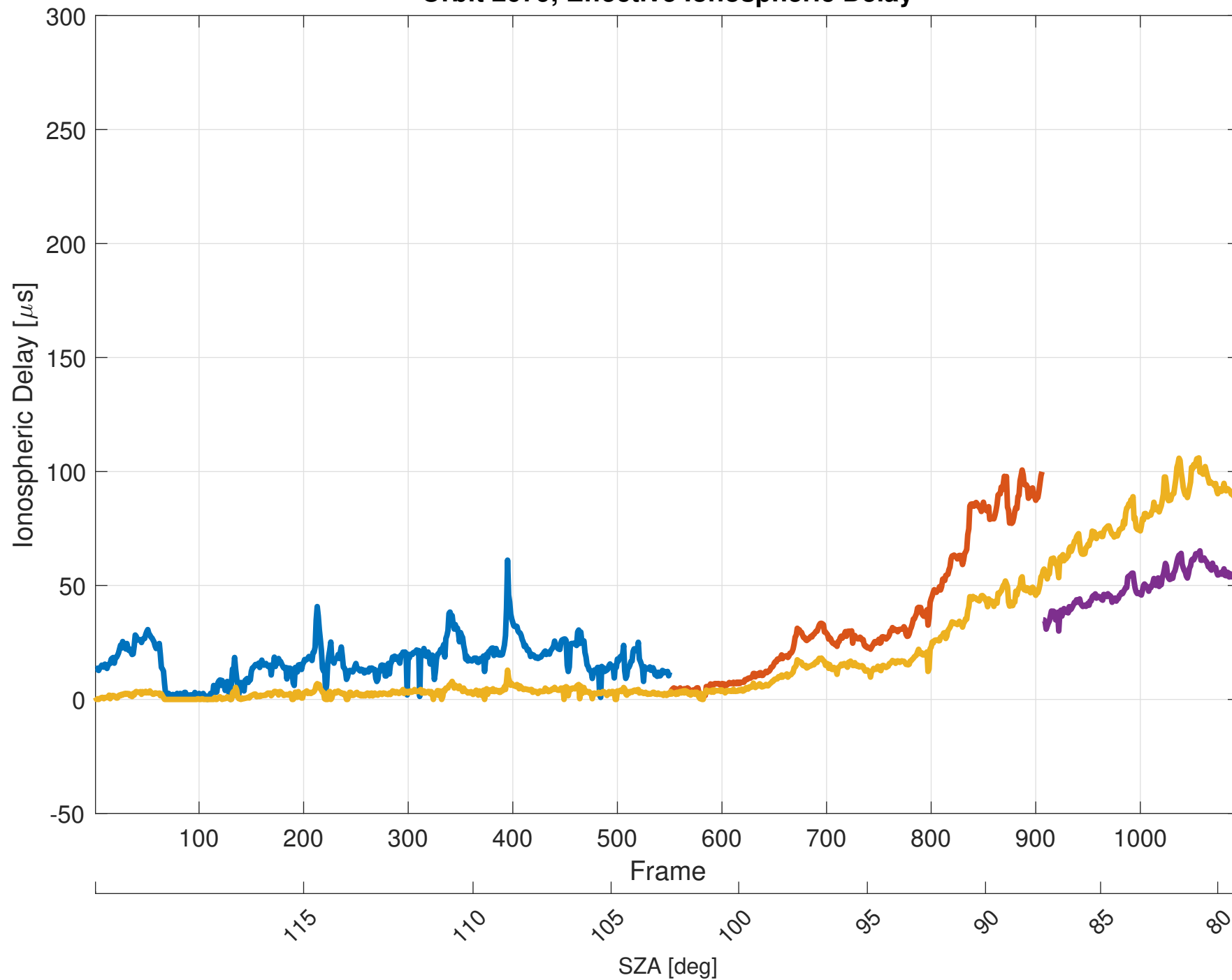
Orbit 2679, Effective Ionospheric Delay
