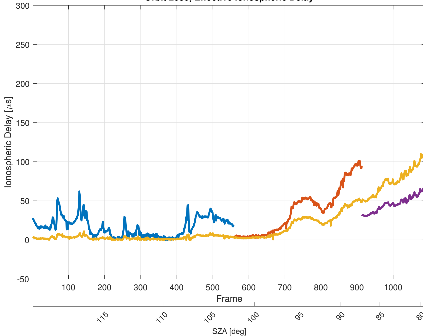
Orbit 2680, Effective Ionospheric Delay
