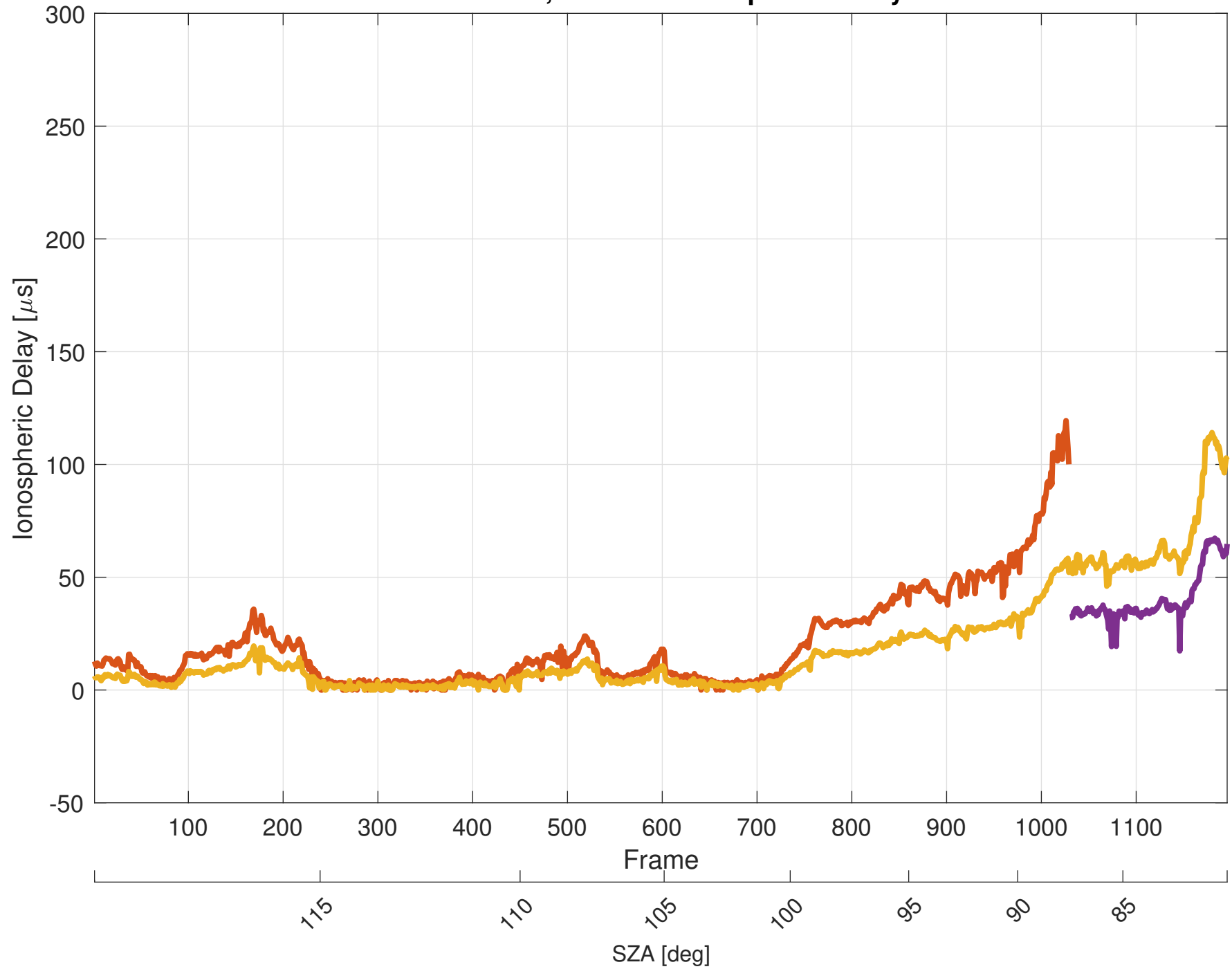
Orbit 2684, Effective Ionospheric Delay
