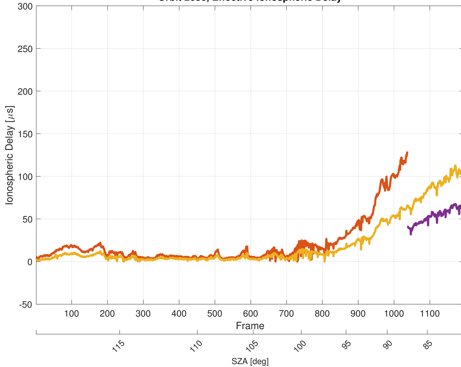
Orbit 2686, Effective Ionospheric Delay
