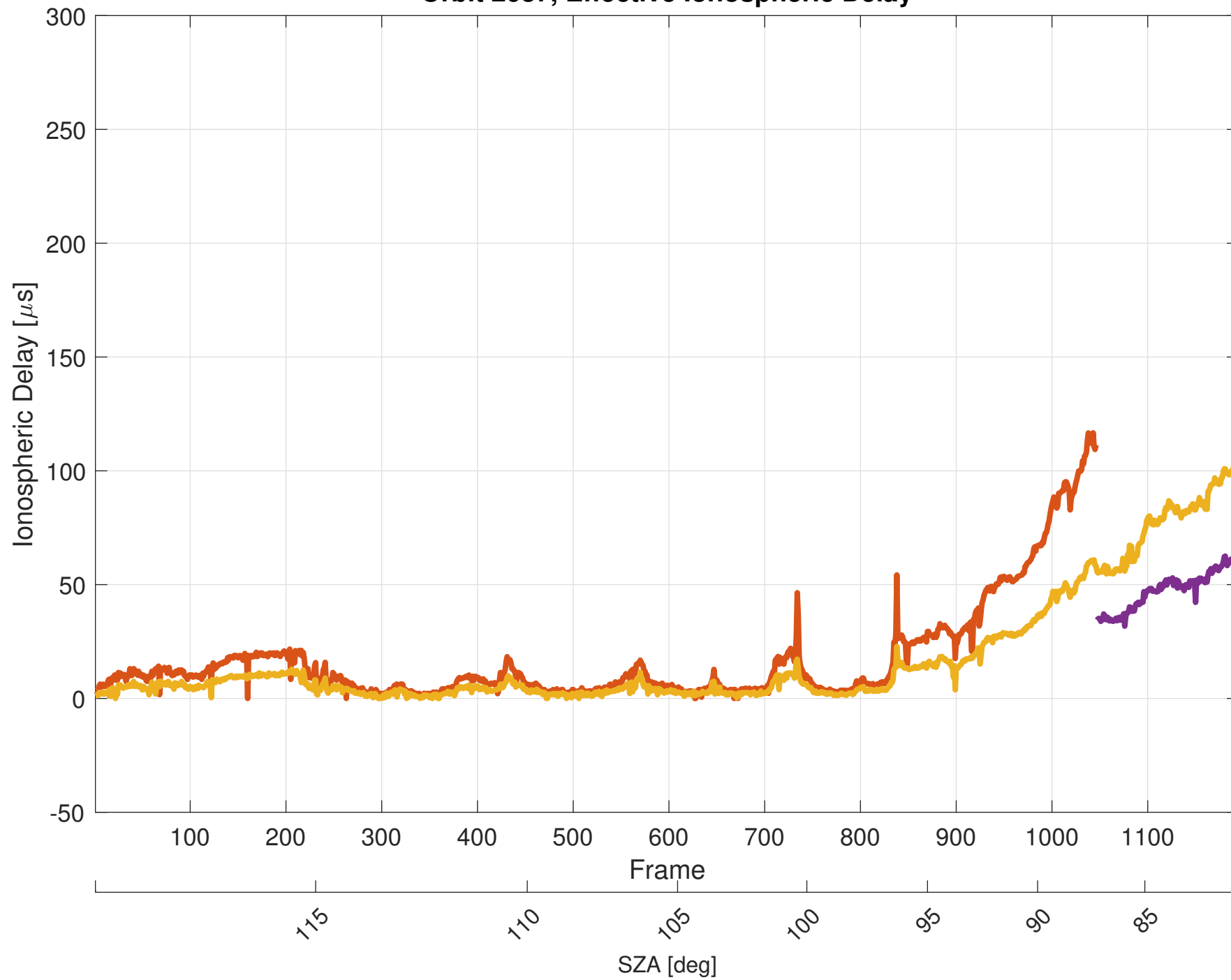
Orbit 2687, Effective Ionospheric Delay
