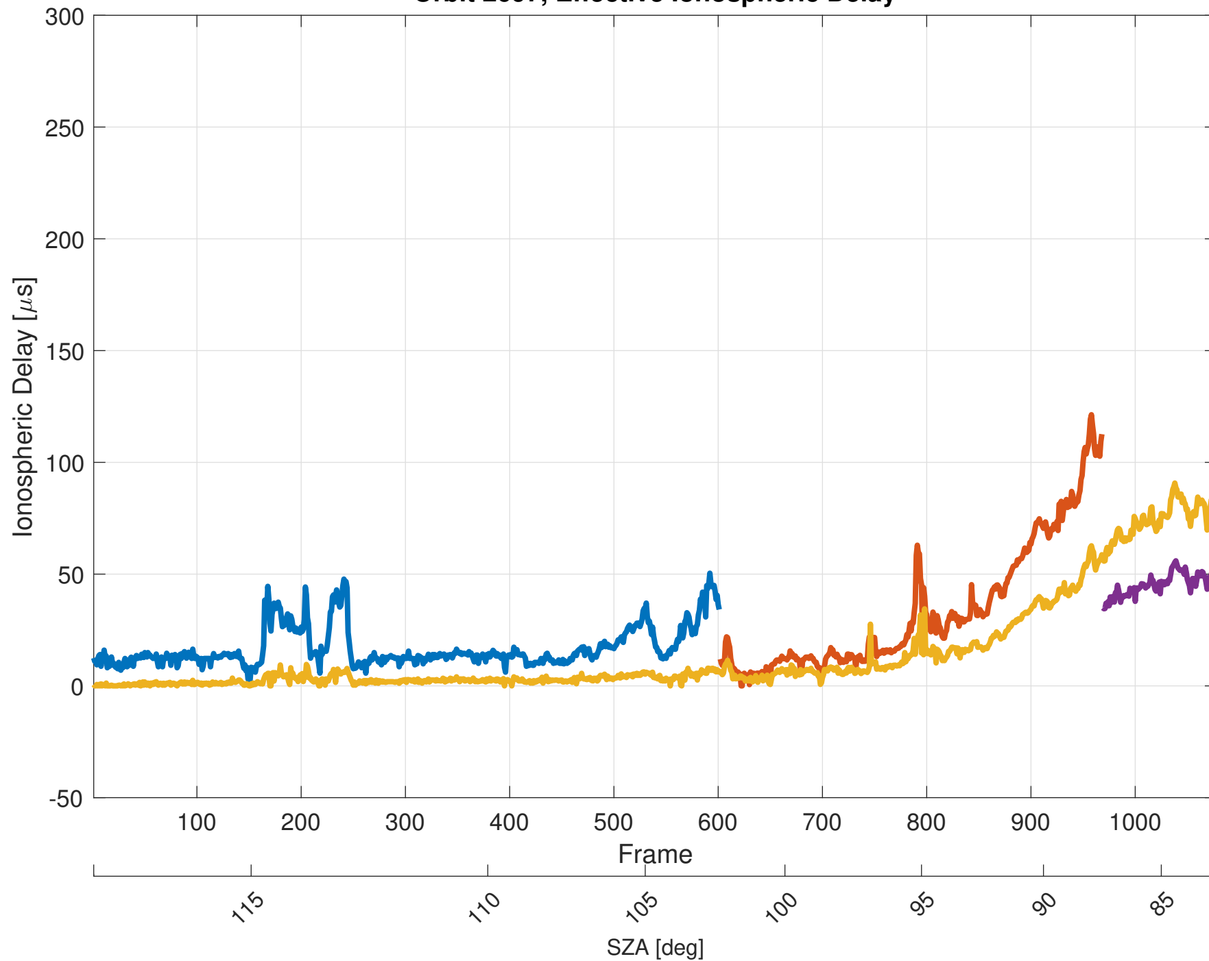
Orbit 2697, Effective Ionospheric Delay
