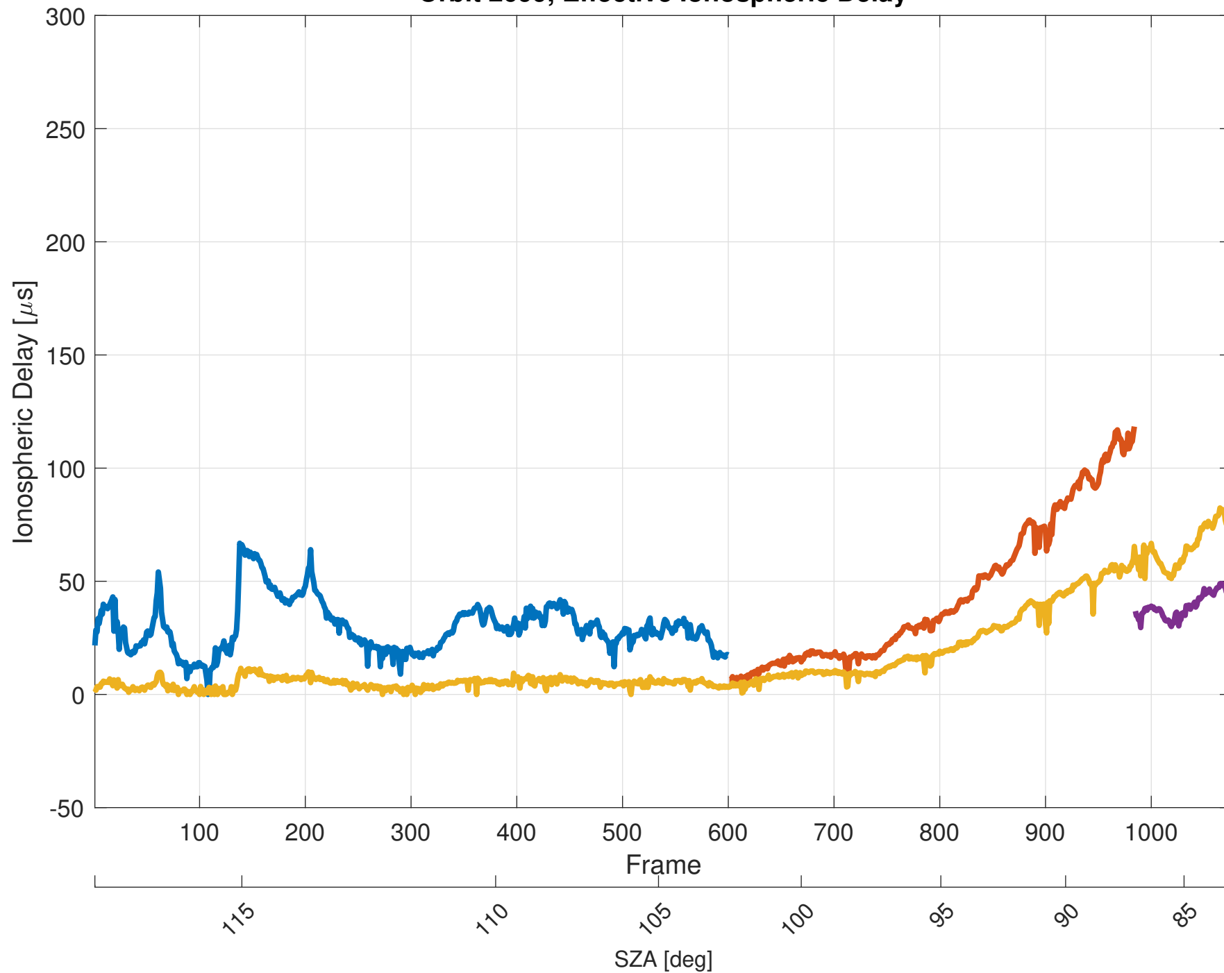
Orbit 2699, Effective Ionospheric Delay
