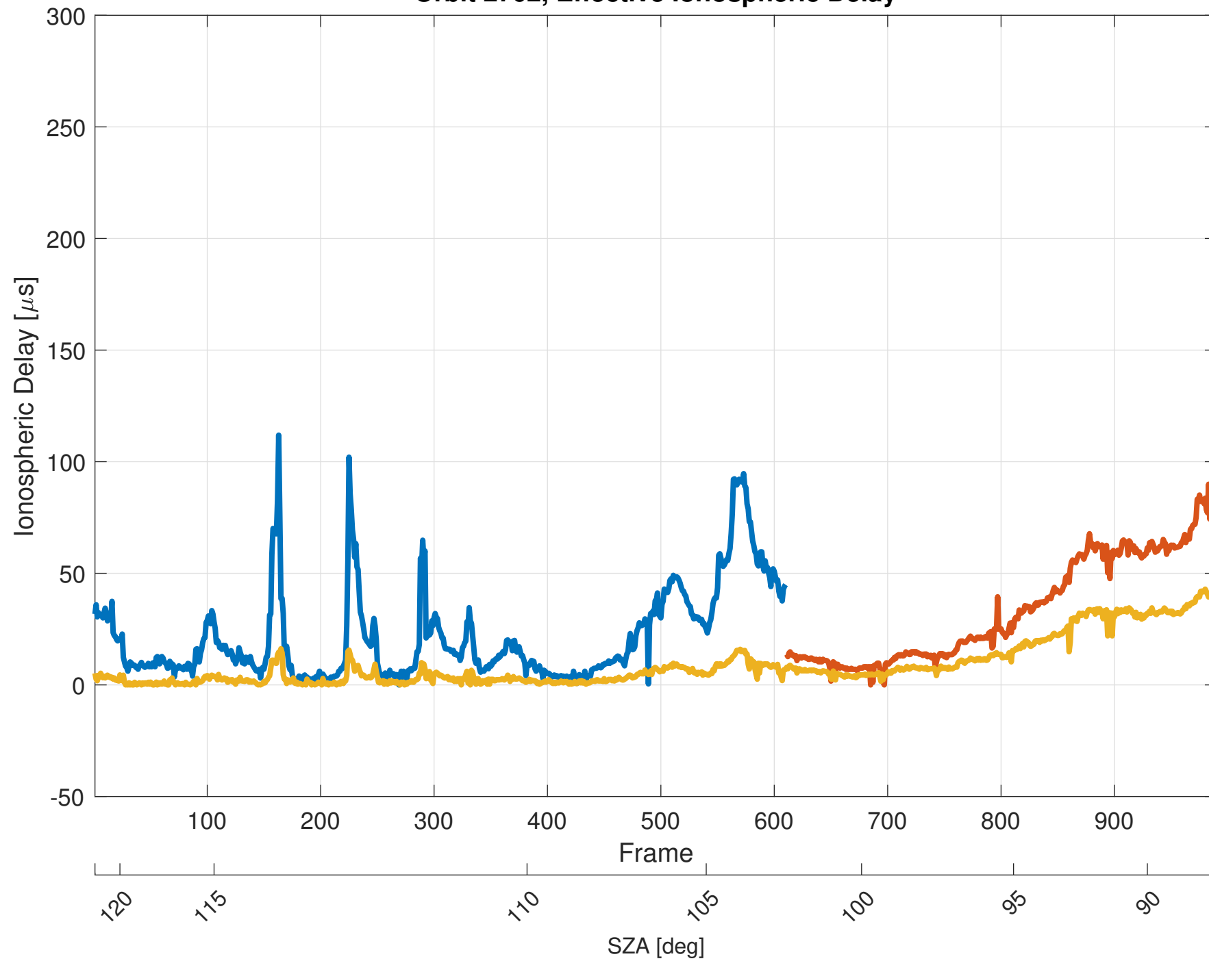
Orbit 2702, Effective Ionospheric Delay
