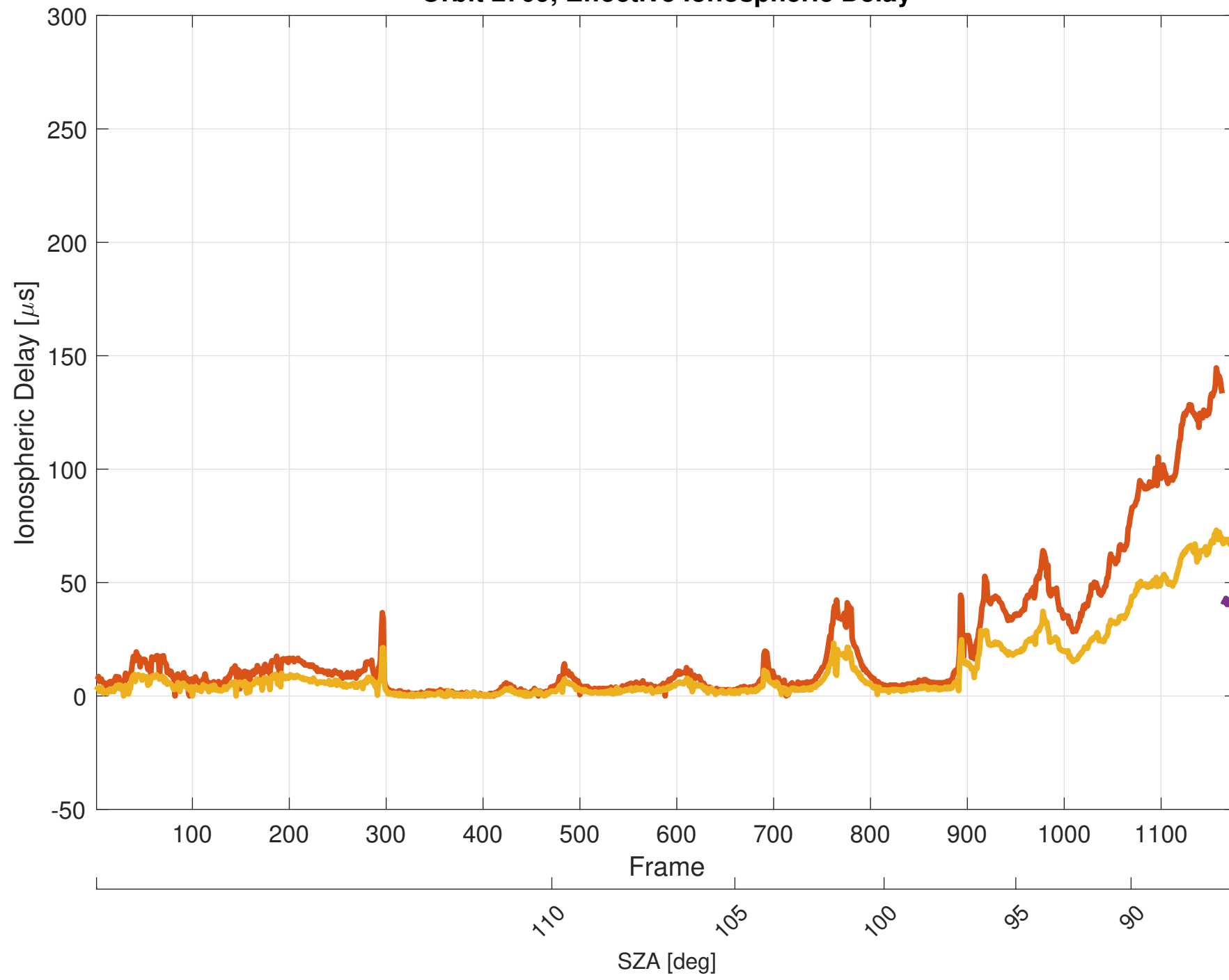
Orbit 2709, Effective Ionospheric Delay
