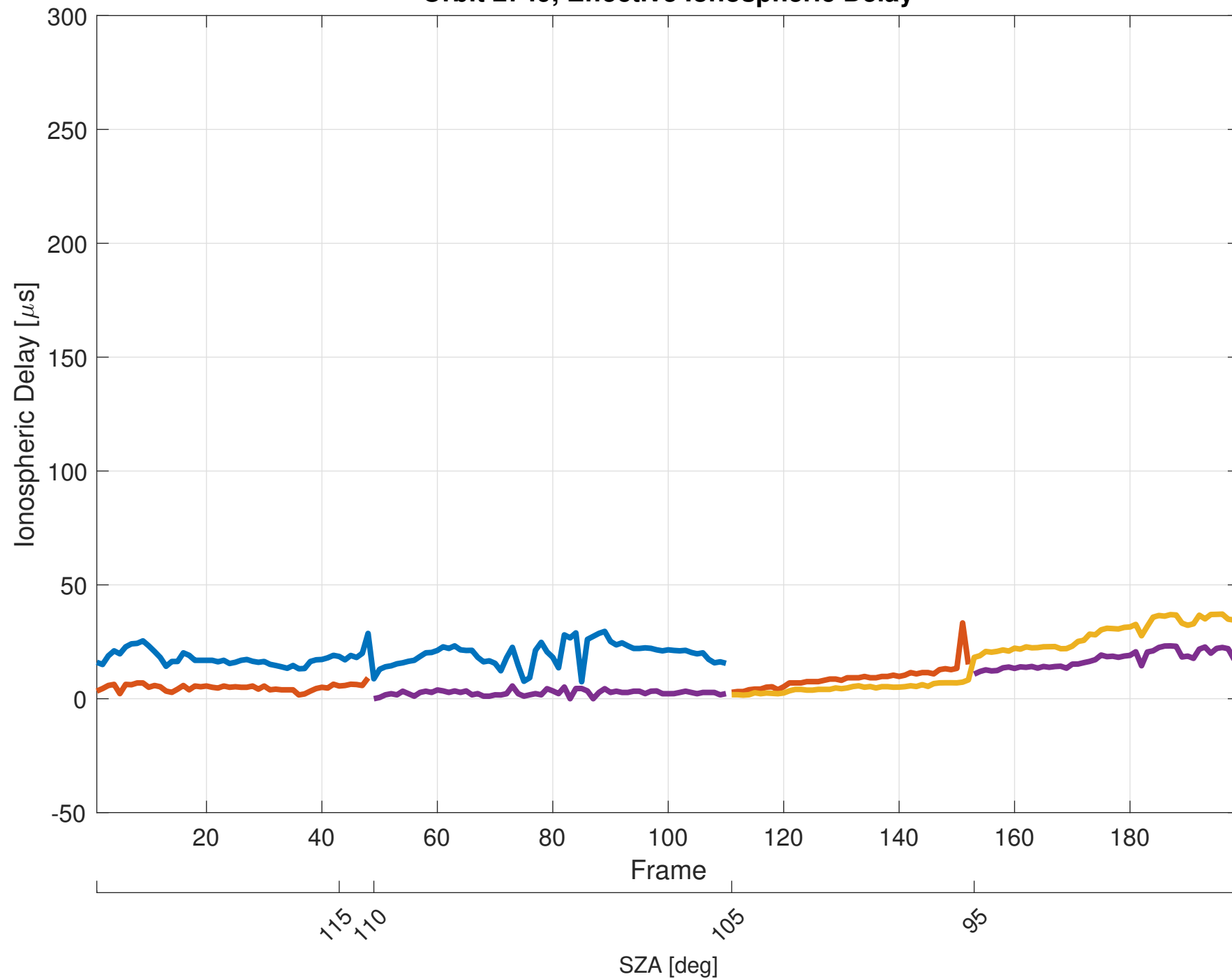
Orbit 2749, Effective Ionospheric Delay
