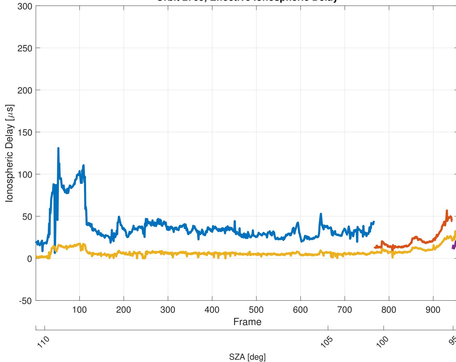
Orbit 2765, Effective Ionospheric Delay
