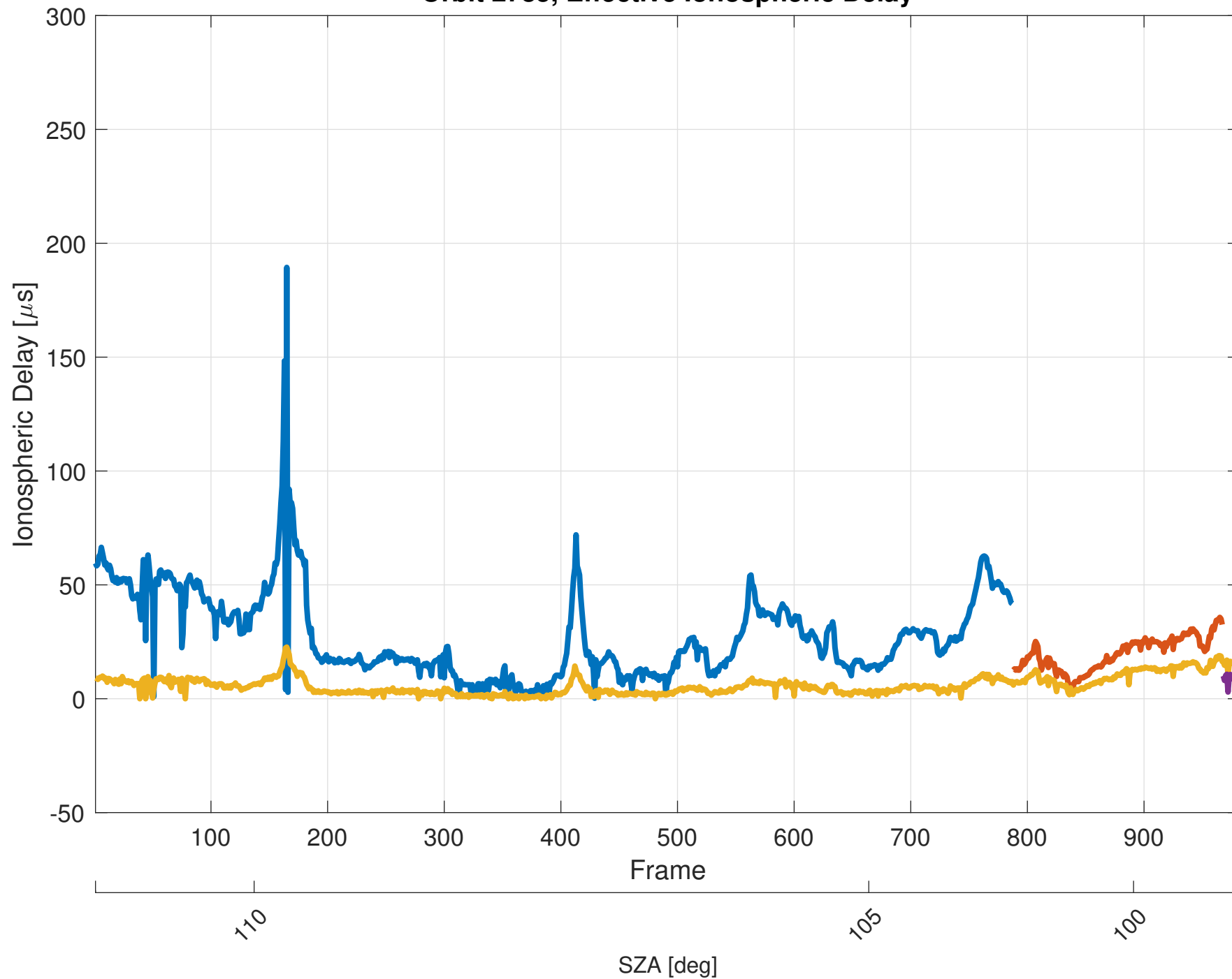
Orbit 2785, Effective Ionospheric Delay
