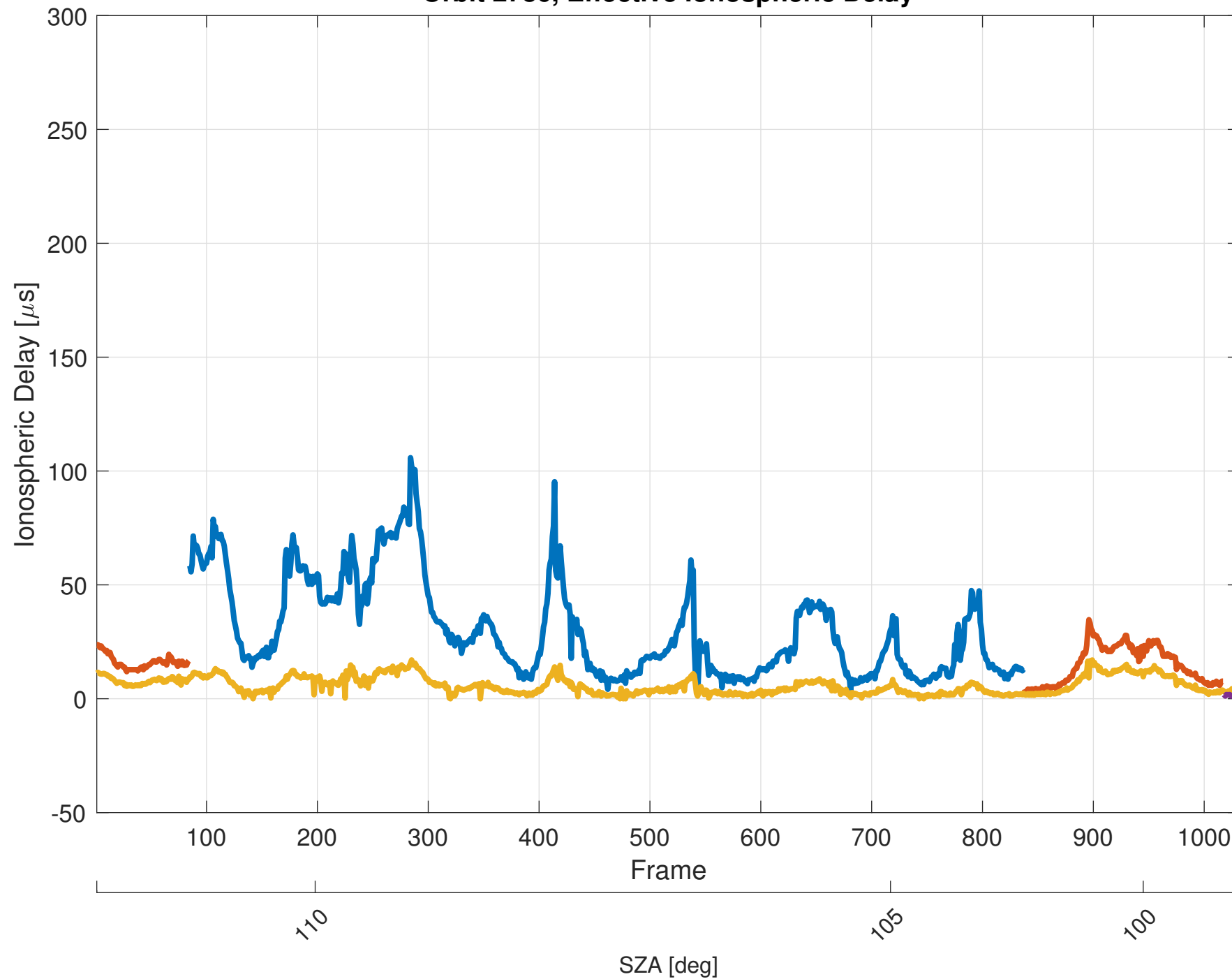
Orbit 2786, Effective Ionospheric Delay
