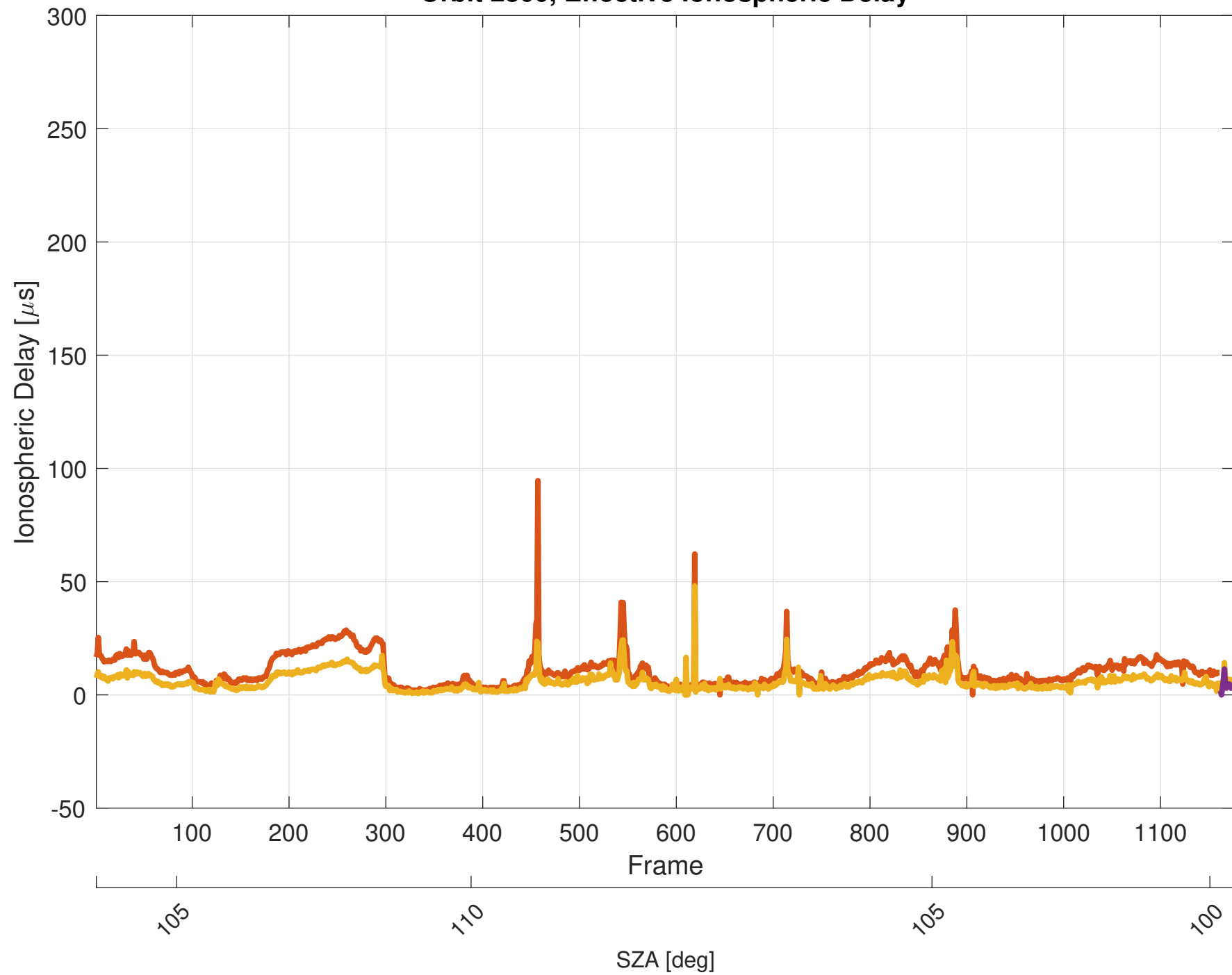
Orbit 2800, Effective Ionospheric Delay
