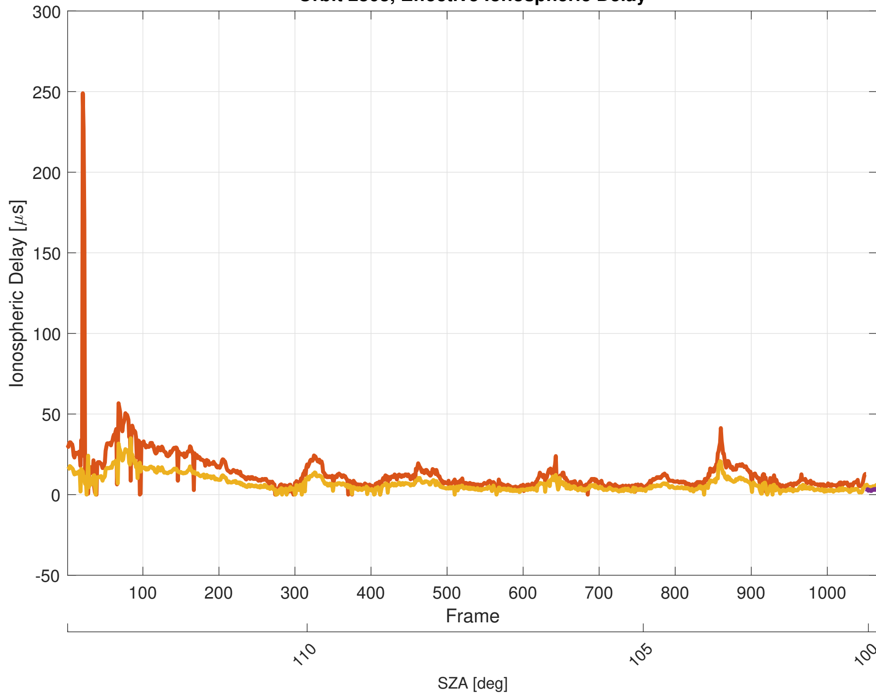
Orbit 2803, Effective Ionospheric Delay
