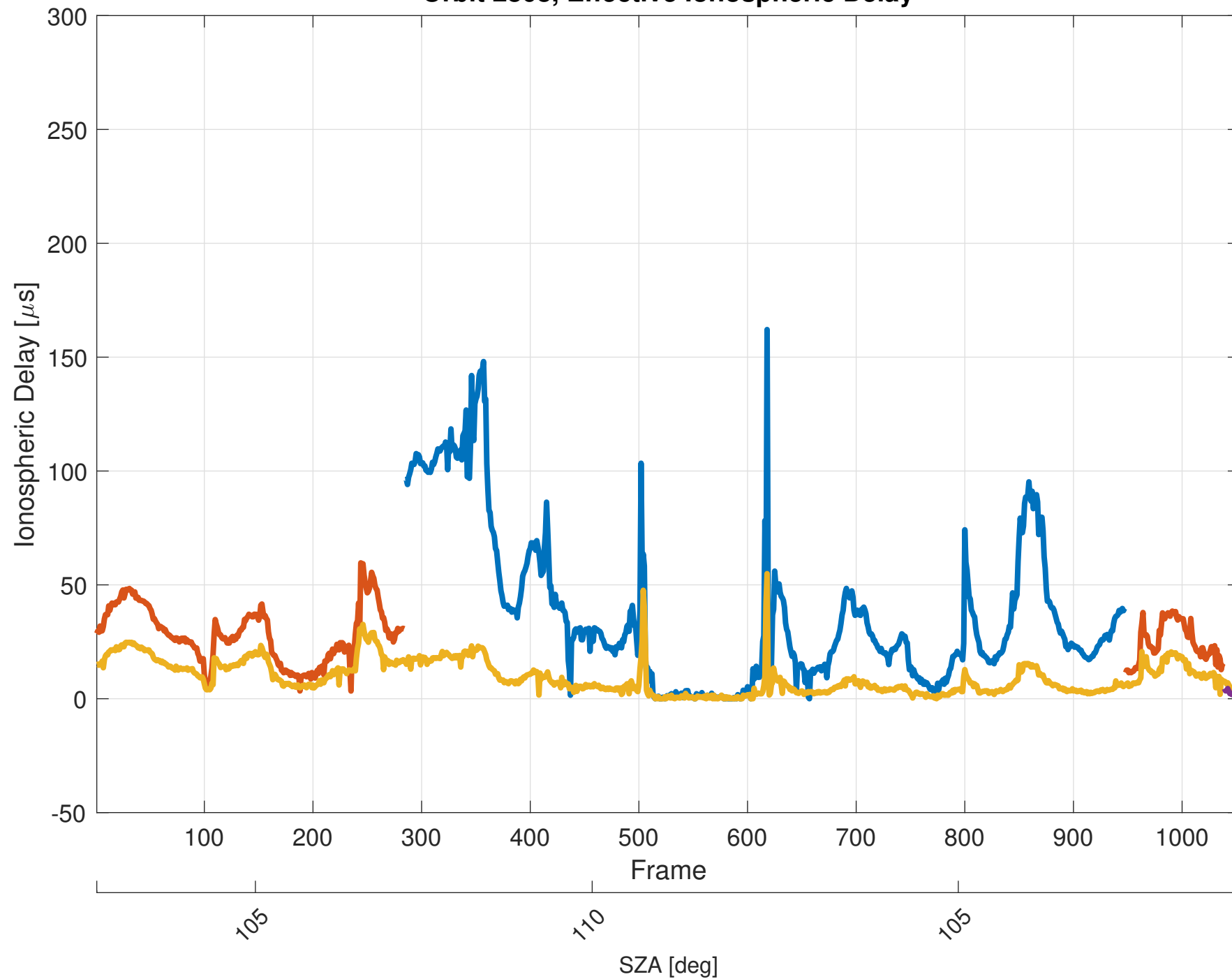
Orbit 2808, Effective Ionospheric Delay
