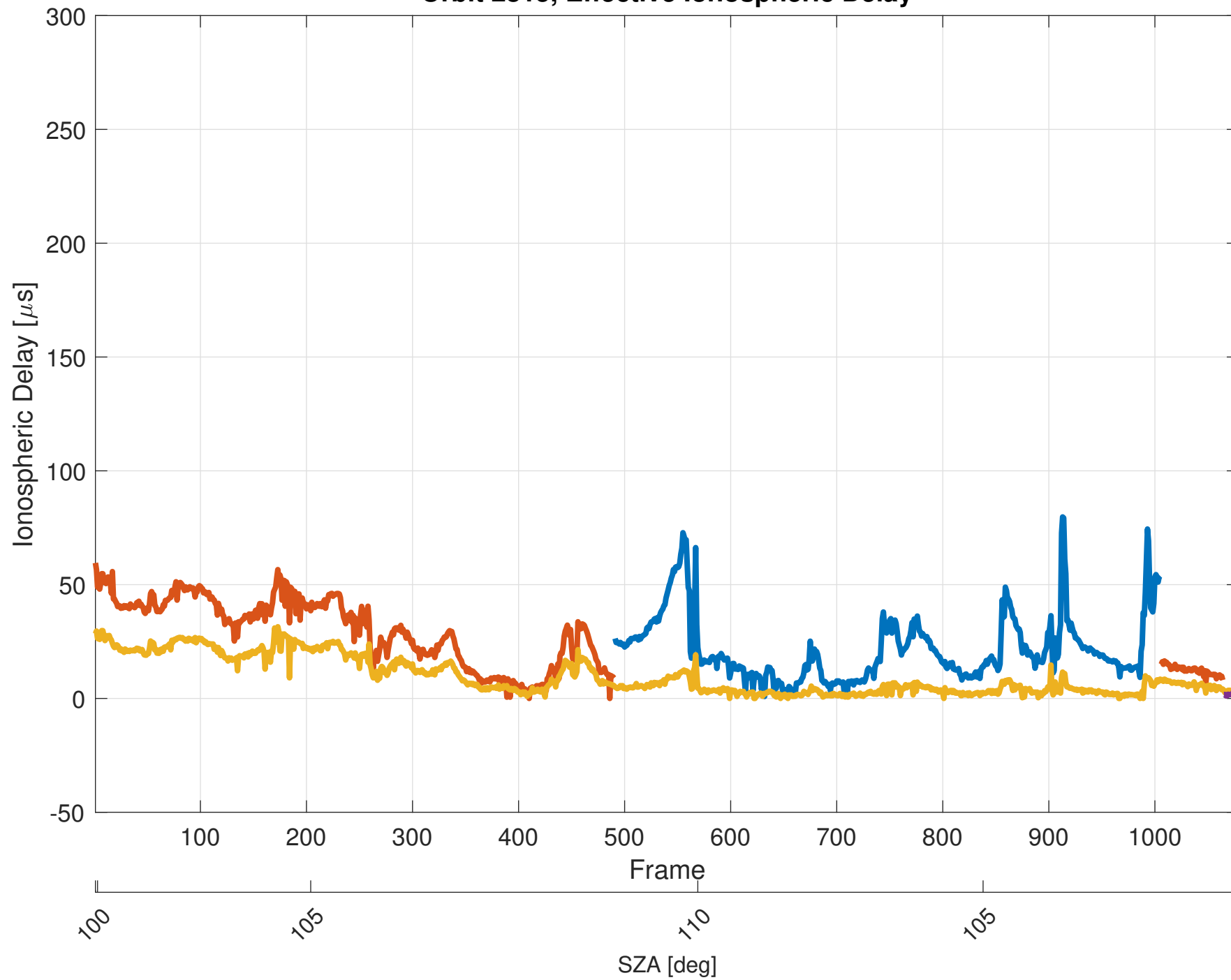
Orbit 2815, Effective Ionospheric Delay
