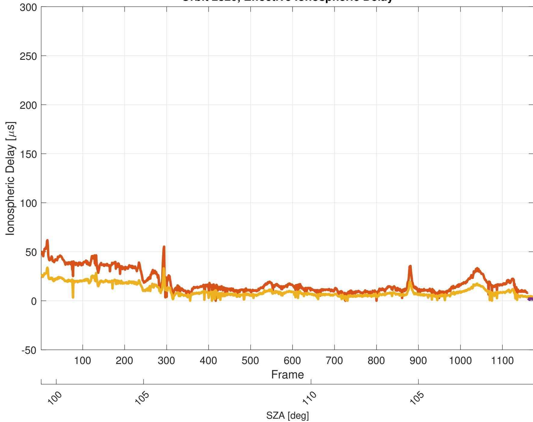
Orbit 2820, Effective Ionospheric Delay
