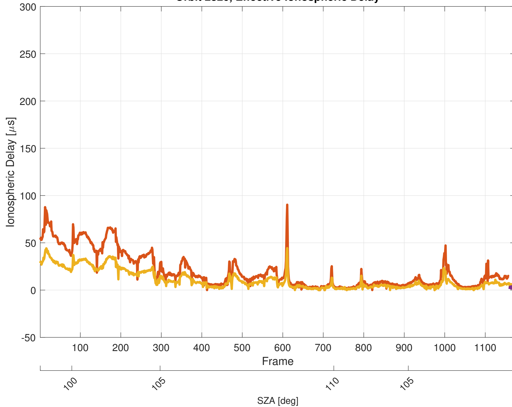
Orbit 2826, Effective Ionospheric Delay
