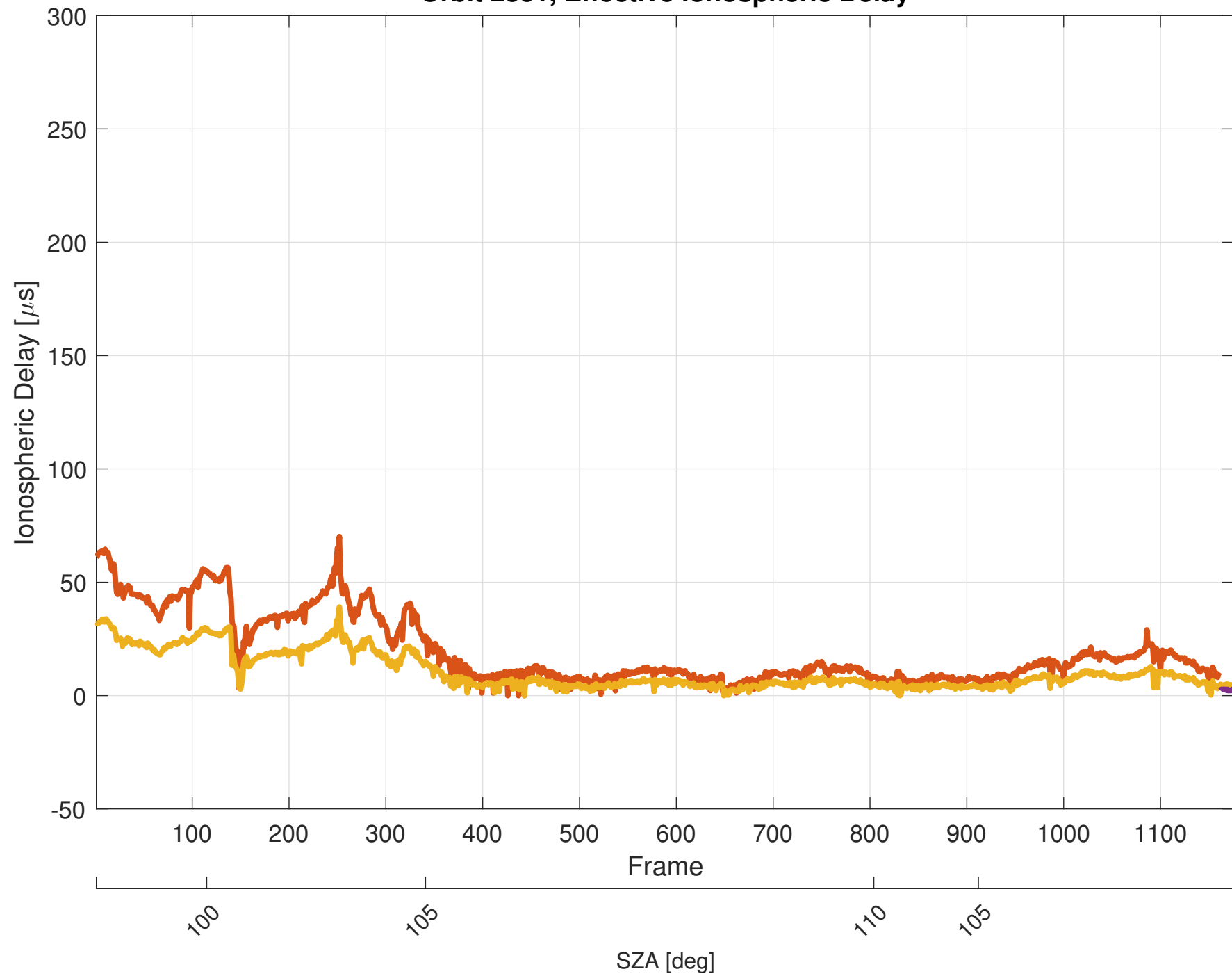
Orbit 2831, Effective Ionospheric Delay
