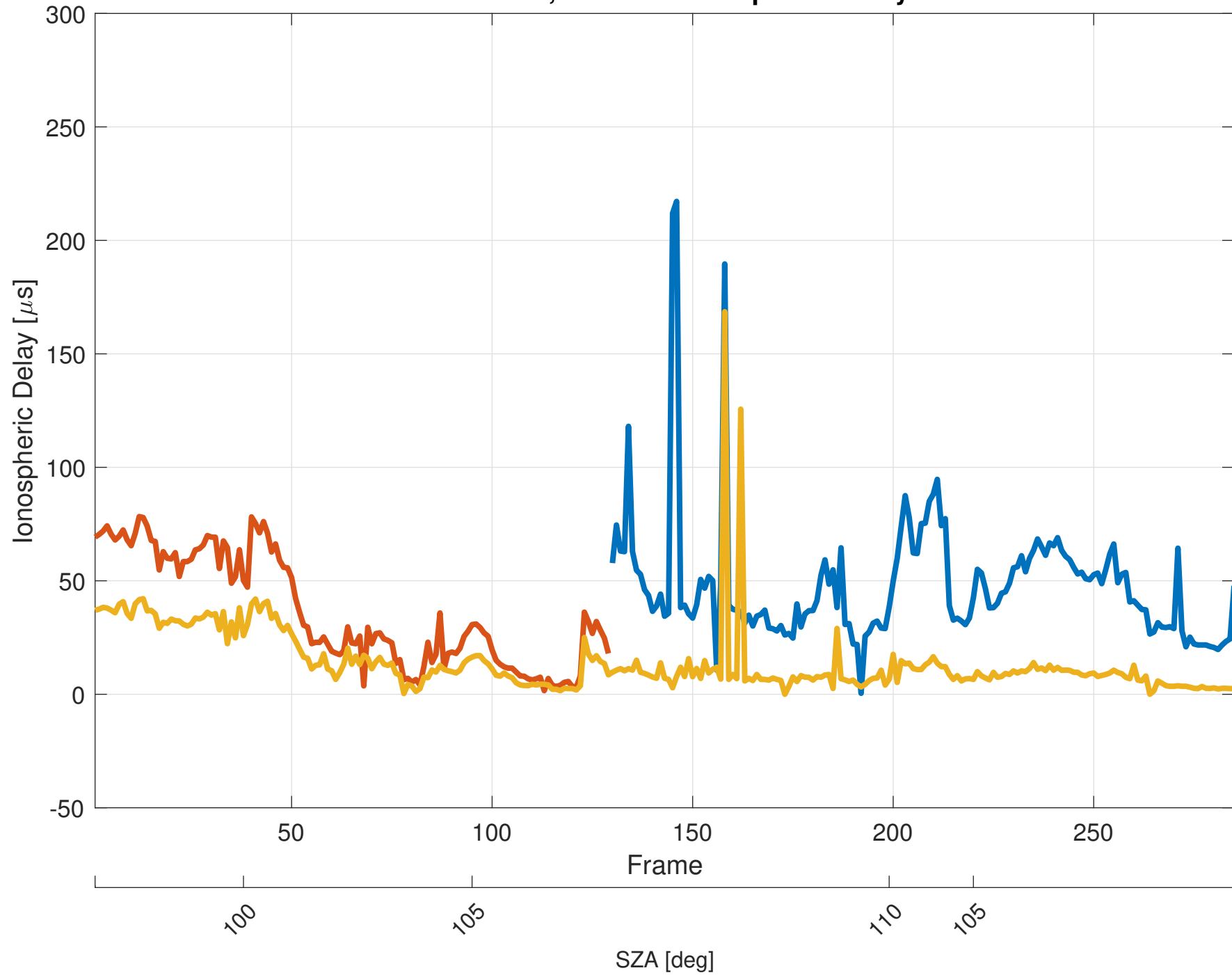
Orbit 2832, Effective Ionospheric Delay
