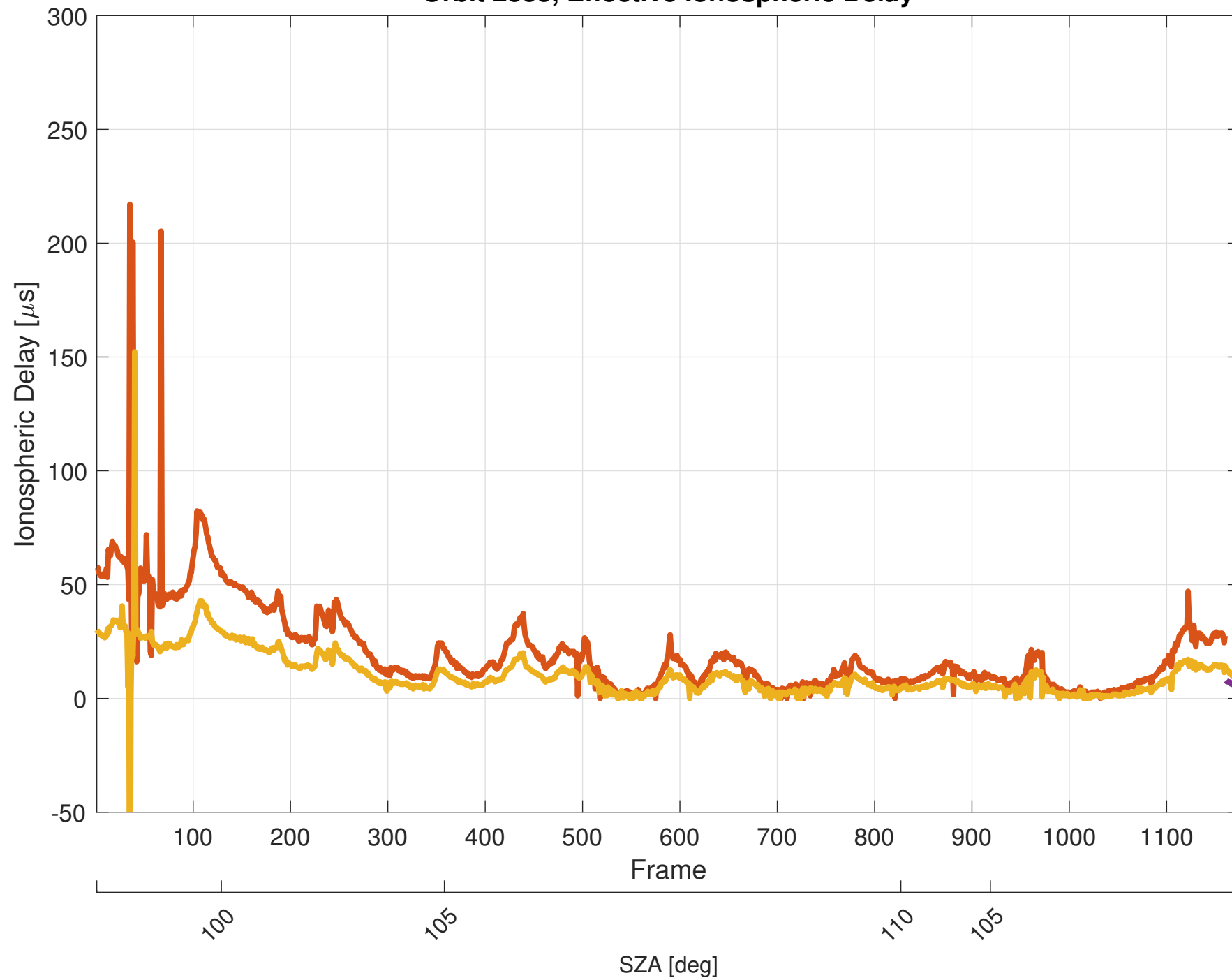
Orbit 2833, Effective Ionospheric Delay
