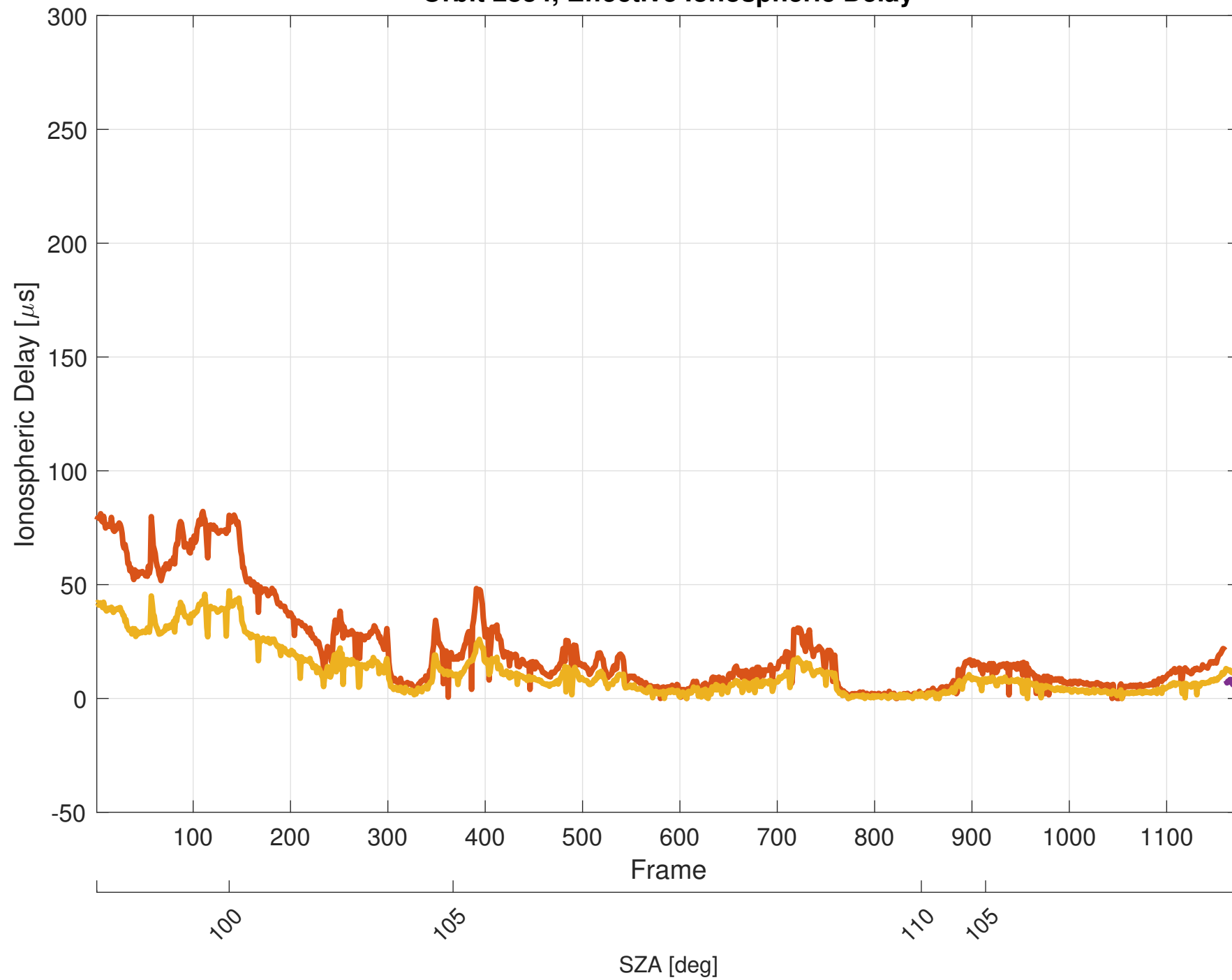
Orbit 2834, Effective Ionospheric Delay
