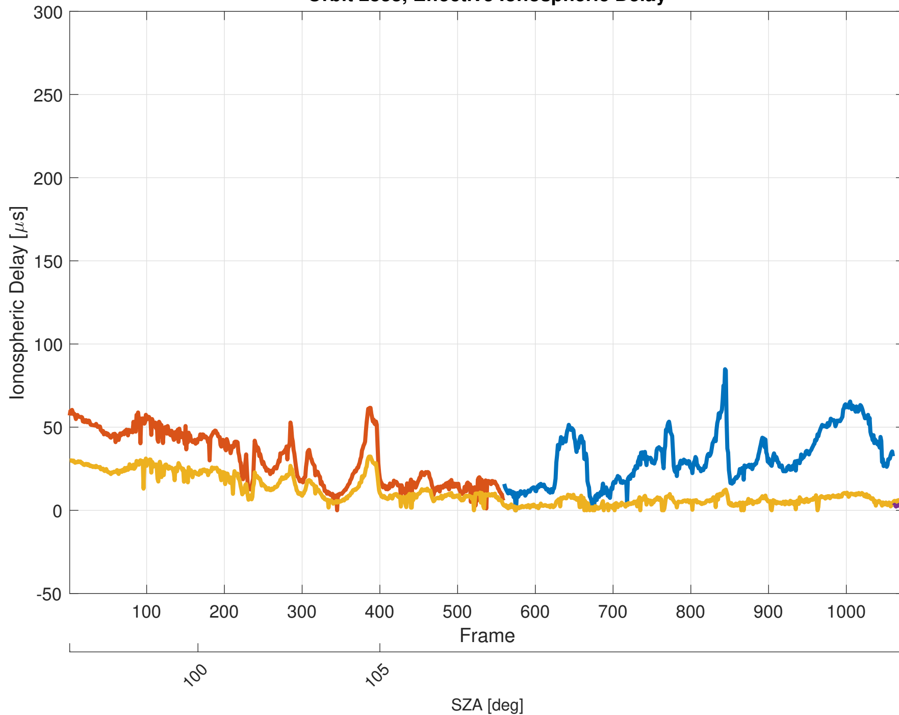
Orbit 2838, Effective Ionospheric Delay
